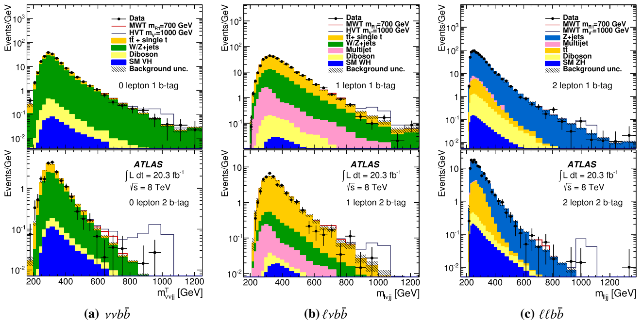
Fig. 1 Distributions of the reconstructed, a transverse mass m_{\nu v_{jj}}^T for the \nu v b \bar{b} final state, b invariant mass m_{\ell \nu_{jj}} for the \ell \nu b \bar{b} final state and c invariant mass m_{\ell \ell_{jj}} for the \ell \ell b \bar{b} final state for the 1- b -tag ( upper ) and 2- b -tag ( lower ) channels. The background expectation is shown after
