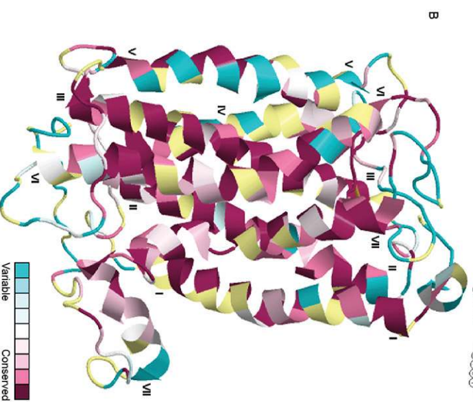
Fig. 2A: conservation pattern of platelet-activating factor (PAF) receptors from 25 animal species. Residues totally conserved among receptors are highlighted in yellow. Multiple sequence alignments were performed using Multiple Sequence Alignment by Log-Expectation (MUSCLE) (Edgar 2004) and the analysis of conserved residues was carried out in Molecular Evolutionary Genetics Analysis (MEGA) 4.0 software (Tamura et al. 2007). The two-dimensional representation of human PAF receptor was adapted from Gui et al. (2007). B: conservation profile for the tertiary structure of PAF receptor (PDB code 2B0X) using ConSurf-conservation analysis. Protein was visualized using FirstGlance in Jmol with colour-coded conservation scores. The conserved and variable residues are coloured according to the conservation scores. Sites, for which the inferred conservation level was assigned with low confidence, are coloured light yellow. Multiple sequence alignments of the 25 PAF receptors were computed using MUSCLE and the Bayesian method (Mayrose et al. 2004) was applied for the calculations of the conservation scores using the Jones-Taylor-Thornton matrix-based method (Jones et al. 1992) as the model of substitution for proteins.
