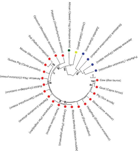
Fig. 1: evolutionary relationships of platelet-activating factor (PAF) receptors from 25 animal species. The evolutionary relationship of PAF receptors was inferred using the neighbour-joining method (Saitou & Nei 1987). The bootstrap consensus tree inferred from 1,000 replicates (Felsenstein 1985) is taken to represent the evolutionary history of the taxa analyzed. The tree is drawn to scale, with branch lengths in the same units as those of the evolutionary distances used to infer the phylogenetic tree. The evolutionary distances were computed using the Jones-Taylor-Thornton matrix-based method (Jones et al. 1992) and are in the units of the number of amino acid (AA) substitutions per site. The analysis involved 25 AA sequences. All positions containing gaps and missing data were eliminated. There was a total of 281 positions in the final dataset. Evolutionary analyses were conducted in Molecular Evolutionary Genetics Analysis 4.0 software (Tamura et al. 2007).
