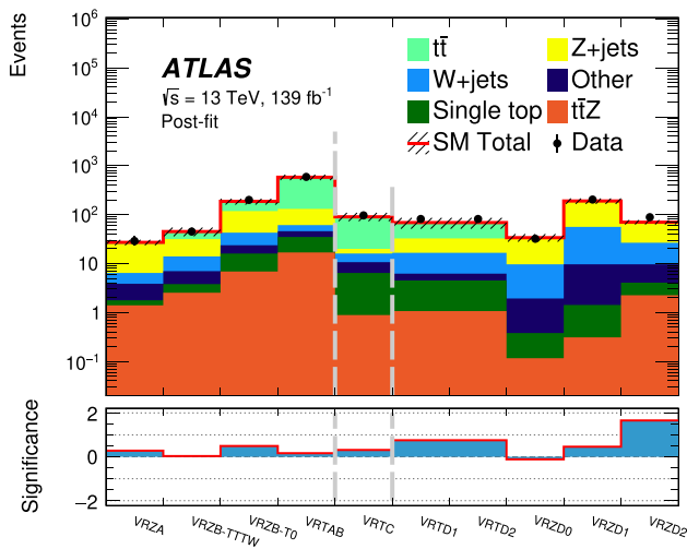
Fig. 10 The total number of data events (points) and the SM expectation (stacked histograms) in all validation regions after the SRA–B, SRC and SRD background-only fits. The stacked histograms show the SM prediction and the hatched uncertainty band around the SM prediction shows the total uncertainty, which includes the MC statistical uncertainties, theory-related and detector-related systematic uncertainties. The lower panel shows the significance of the difference between data and the background prediction calculated with the method described in Ref. [122]. The validation regions considered in the SRA–B, SRC and SRD fits are separated by vertical dashed lines
