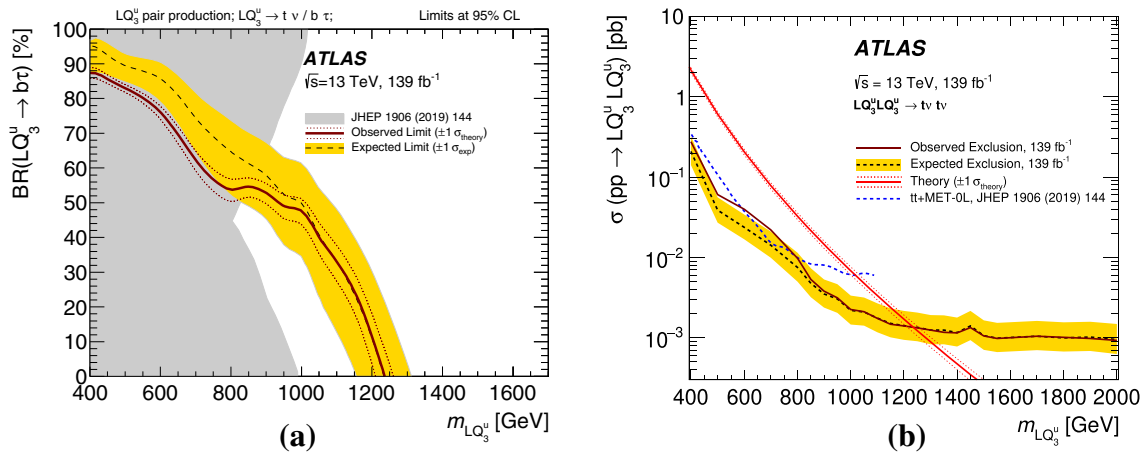
Fig. 14 Observed (red solid line) and expected (black dashed line) limits on up-type, third-generation leptoquarks. a Limits as a function of the branching ratio of leptoquarks decaying into b\tau (with the only other decay allowed being into t\nu ) vs leptoquark mass. b Limits on the production cross section at 95% CL as a function of leptoquark mass
