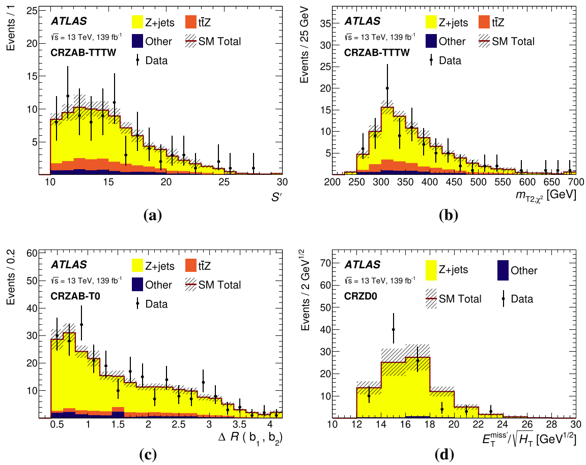
Fig. 4 Distributions illustrating the level of agreement between data (points) and the SM expectation (stacked histograms, after simultaneously fitting to all backgrounds) in several Z + jets control regions: a S' and b m_{T2,\chi^2} for CRZAB-TTTW, c \Delta R(b_1, b_2) for CRZAB-T0, and d
