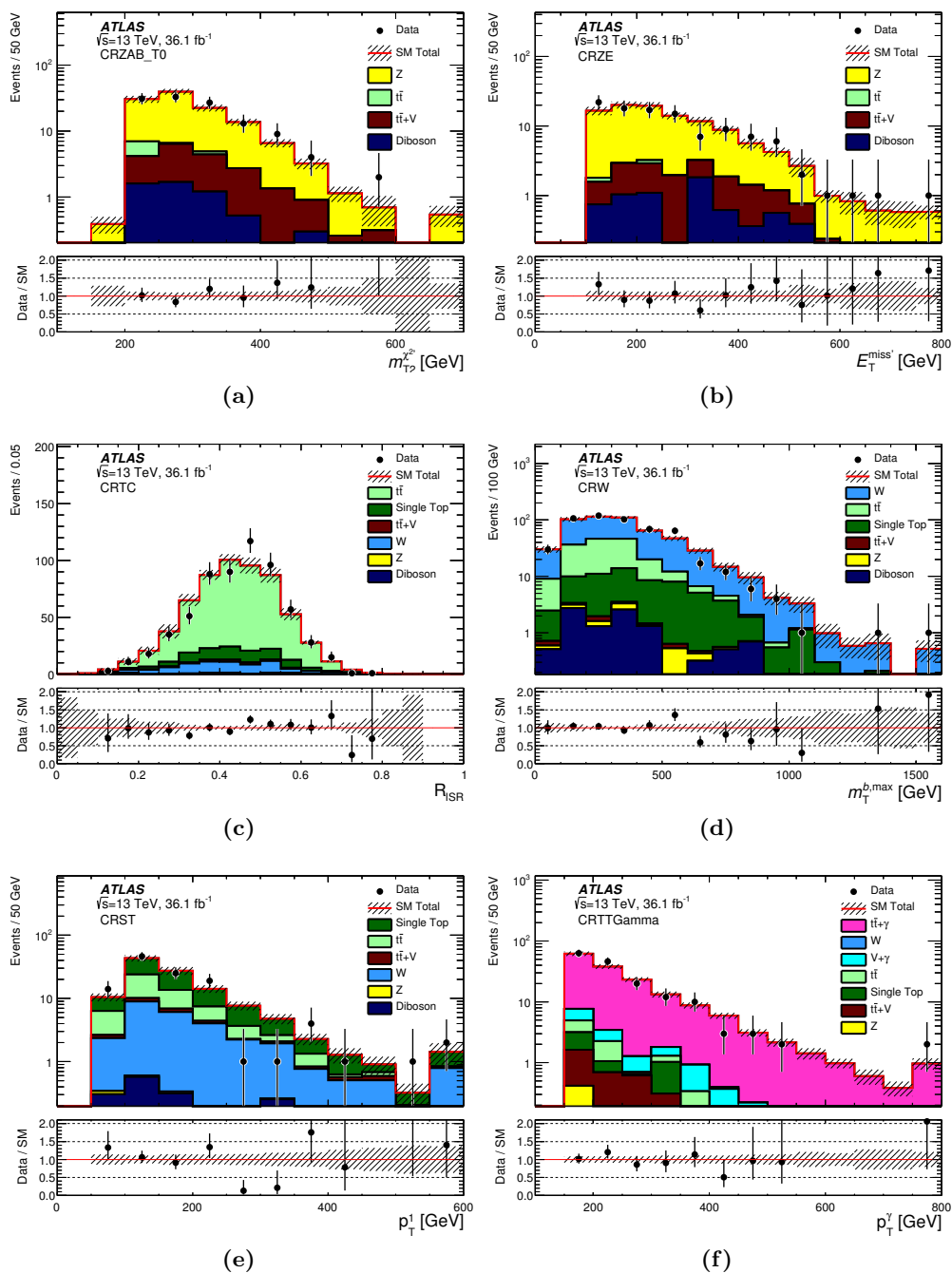
Figure 4. Distributions of (a) m_{T2}^{\chi_{2'}} in CRZAB-T0, (b) E_T^{miss'} in CRZE, (c) R_{ISR} in CRTC, (d) m_T^{b,max} in CRW, (e) the transverse momentum of the second-leading- p_T jet in CRST, and (f) the photon p_T in CRTTGamma. The stacked histograms show the SM prediction, normalized using scale factors derived from the simultaneous fit to all backgrounds. The “Data/SM” plots show the ratio of data events to the total SM prediction. The hatched uncertainty band around the SM prediction and in the ratio plot illustrates the combination of MC statistical and detector-related systematic uncertainties. The rightmost bin includes overflow events.
