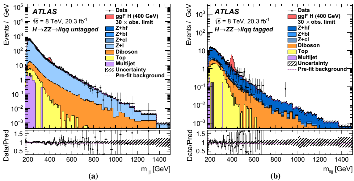
Fig. 3 The distributions used in the likelihood fit of the invariant mass of dilepton + dijet system m_{\ell\ell jj} for the H \rightarrow ZZ \rightarrow \ell^+ \ell^- q\bar{q} search in the a untagged and b tagged resolved ggF subchannels. The dashed line shows the total background used as input to the fit. The simulated signal
