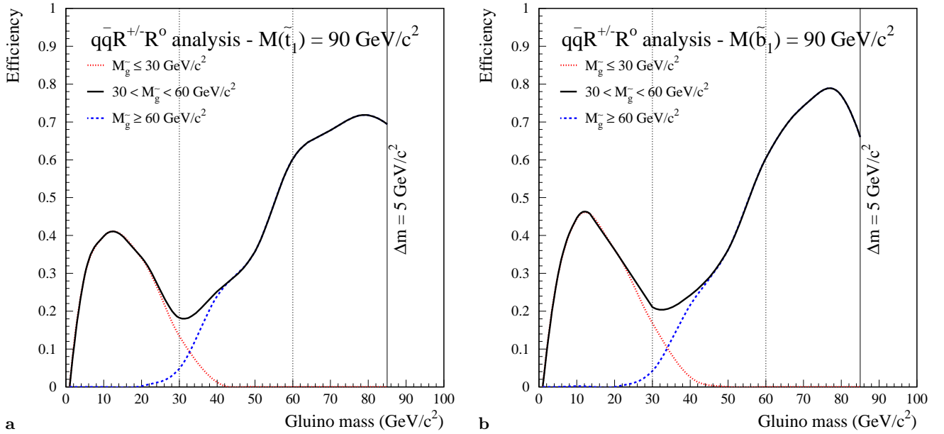
Fig. 12a,b. Signal detection efficiencies at \sqrt{s}=200 GeV for the stop a and sbottom b q\bar{q}R^{\pm}R^{\circ} analysis as a function of the gluino mass ( m_{\tilde{q}_1} = 90 GeV/c 2 ). \Delta M is the mass difference between the squark and the gluino. Vertical lines show the limits of the mass analysis window. The last one ends at \Delta M = 5 GeV/c 2 which corresponds the last simulated signal points
