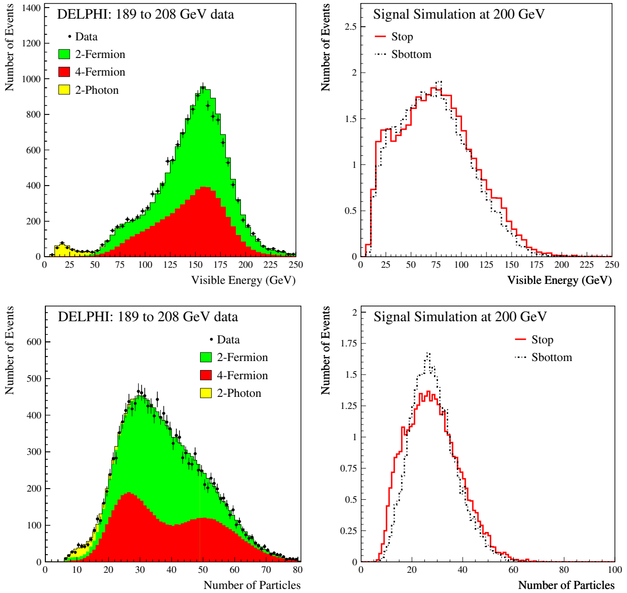
Fig. 13. Data-simulation comparison at the preselection level of the LEP2 q\bar{q}R^\circ R^\circ analysis. Data taken in the centre-of-mass energy range between 189 and 208 GeV were included. Right-hand side histograms show the expected distributions with arbitrary normalization for the stop and the sbottom signal at 200 GeV when all simulated samples are added together
