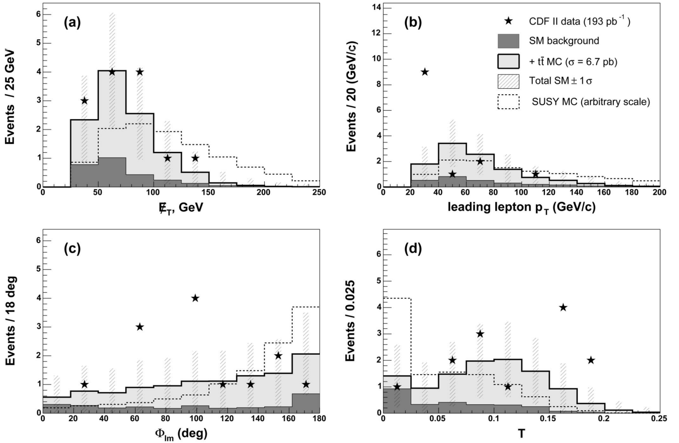
FIG. 1. \cancel{E}_T , leading lepton p_T , \Phi_{\ell m} , and T distributions for the top dilepton sample. The hatched regions represent the Poisson uncertainty on the expectation in a given bin. The dashed histograms are the expected distributions from the SUSY MC calculation described in the text.
