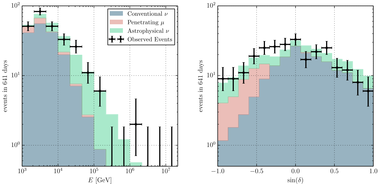
Figure 1. Reconstructed energy (left) and declination (right) distributions for the best-fit atmospheric and astrophysical spectra (shaded histograms) obtained in Aartsen et al. (2015b) compared to the distributions for the 263 cascades (black crosses) depositing at least 1 TeV observed in that analysis. Atmospheric muons misidentified as cascades after passing undetected through the veto layer are concentrated at \sin(\delta) < -0.3 , while in the same range some atmospheric neutrinos are rejected because they are accompanied by incoming muons.
