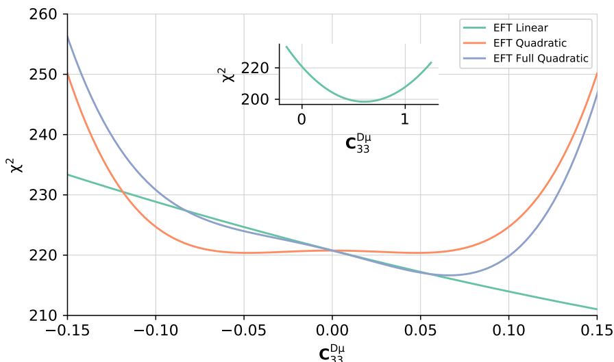
Figure 8. The results of polynomial fits to \chi^2(C_{33}^{D\mu}) , eq. (4.2), in scenario II. This \chi^2 includes only the contributions from the two DY measurements in the dimuon final state. We display results for fits based on cross sections that account only for the linear, only for the quadratic, and for both linear and quadratic terms in the EFT expansion, in all cases using the baseline SM PDF set. The inset displays the fit to the linear EFT values with an enlarged x -axis range.
