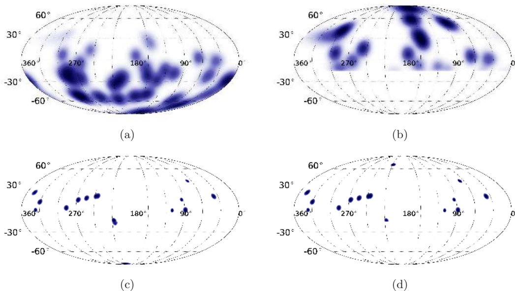
Figure 5. Neutrino likelihood maps convoluted with the exposures of the CR Observatories in Equatorial coordinates. The two upper plots are for the high-energy cascades, while the two lower ones are for the high-energy tracks. The declination-dependent exposure of Auger is applied in (a) and (c) and that of TA in plots (b) and (d).
