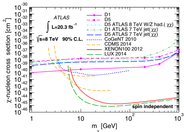
FIG. 6 (color online). Observed 90% C.L. upper limits on the \chi -nucleon scattering cross section as a function of m_\chi for spin-independent effective operators mediating the interaction of the dark-matter particles with the q\bar{q} initial state. The limits are compared with results from the published ATLAS hadronically decaying W/Z [8] and j + \chi\chi [4] searches, CoGeNT [42], XENON100 [43], CDMS [44,45], and LUX [46]. These limits are shown as they are given in the corresponding publications and are only shown for comparison with the results from this analysis, since they are obtained assuming the interactions are mediated by operators different from those used for the ATLAS limits.
