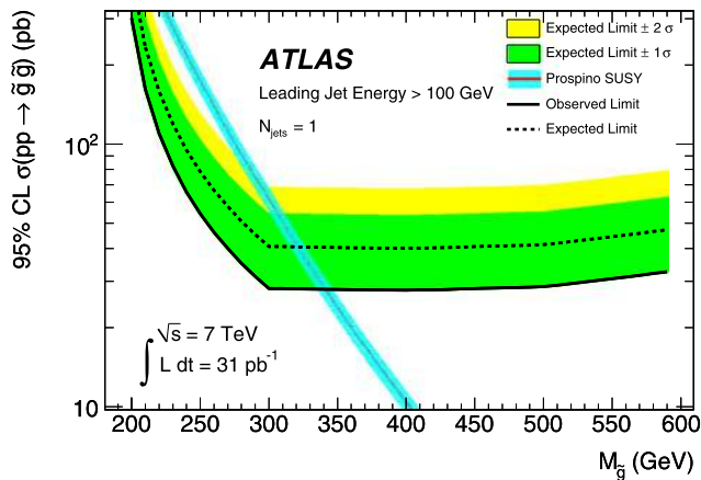
Fig. 4 The 95 % C.L. limit on the gluino pair production cross-section as a function of gluino mass, m_{\tilde{g}} , assuming m_{\tilde{\chi}_1^0} = 100 GeV. Limits are shown for the Generic stopping model and \tilde{g} \rightarrow g\tilde{\chi}^0 decay
