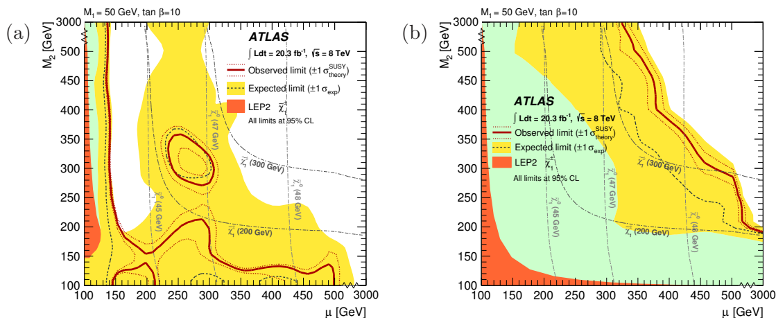
Figure 10. (a) 95% CL exclusion regions in the \mu - M_2 mass plane of the pMSSM with very large slepton masses, M_1 = 50 GeV and \tan\beta = 10 . (b) The exclusion region obtained by combining the results from SR-Zjets with those from the ATLAS three-lepton search [83]. The areas covered by the -1\sigma expected limit are shown in green. The dash-dotted lines indicate the masses of \tilde{\chi}_1^\pm and \tilde{\chi}_1^0 . Also shown are the LEP limits [36, 37] on the mass of the chargino.
