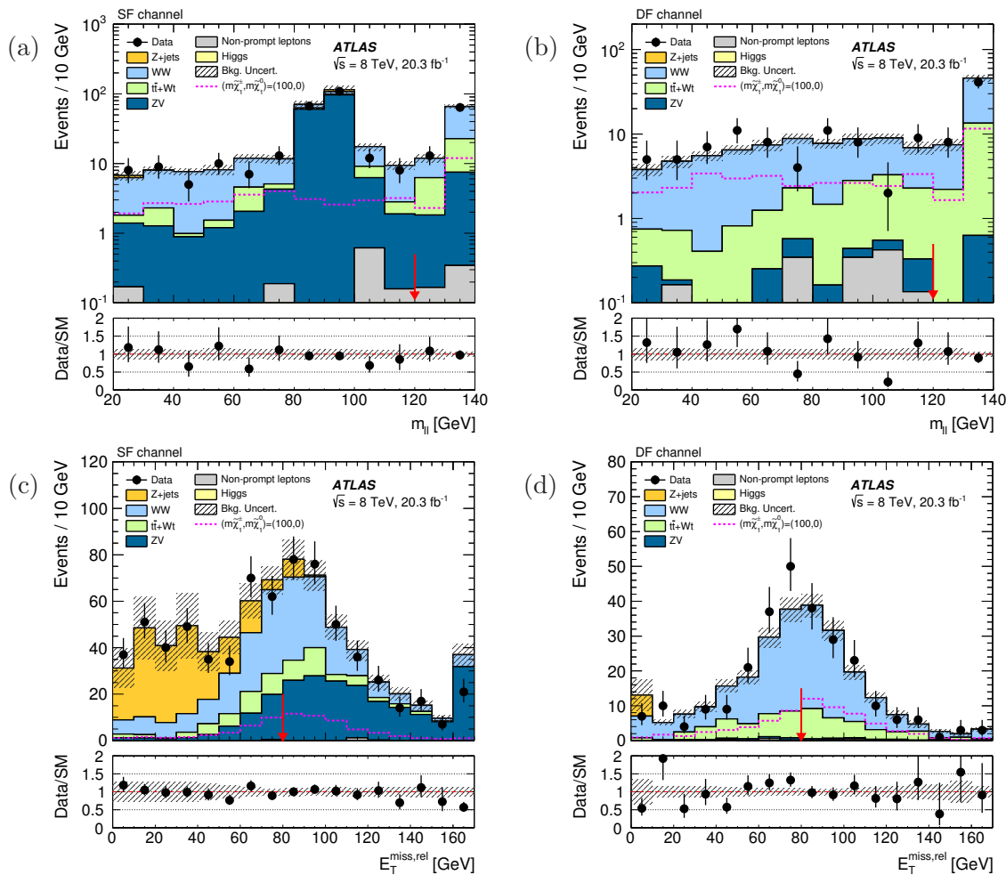
Figure 3. Distributions of m_{\ell\ell} in the (a) SF and (b) DF samples that satisfy all the SR- WWa selection criteria except for the one on m_{\ell\ell} , and of E_T^{\text{miss,rel}} in the (c) SF and (d) DF samples that satisfy all the SR- WWa selection criteria except for the ones on m_{\ell\ell} and E_T^{\text{miss,rel}} . The lower panel of each plot shows the ratio between data and the SM background prediction. The hashed regions represent the sum in quadrature of systematic uncertainties and statistical uncertainties arising from the numbers of MC events. Predicted signal distributions in a simplified model with m_{\tilde{\chi}_1^\pm} = 100 GeV and m_{\tilde{\chi}_1^0} = 0 are superimposed. Red arrows indicate the SR- WWa selection criteria. In (a), the region 81.2 < m_{\ell\ell} < 101.2 GeV is rejected by the Z boson veto.
