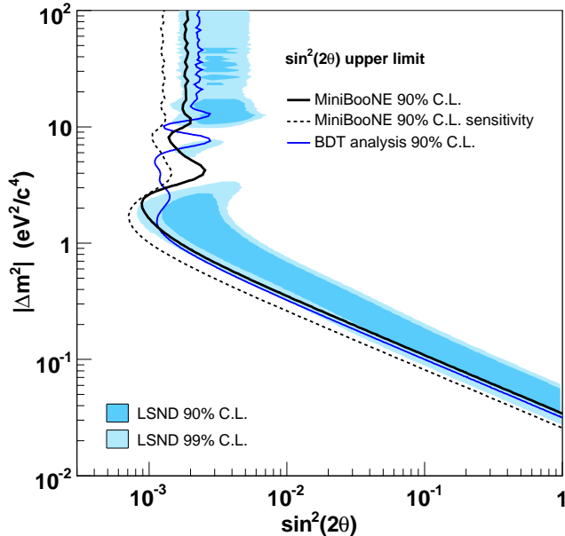
FIG. 3: The MiniBooNE 90% CL limit (thick solid curve) and sensitivity (dashed curve) for events with 475 < E_\nu^{QE} < 3000 MeV within a two neutrino oscillation model. Also shown is the limit from the boosted decision tree analysis (thin solid curve) for events with 300 < E_\nu^{QE} < 3000 MeV. The shaded areas show the 90% and 99% CL allowed regions from the LSND experiment.
