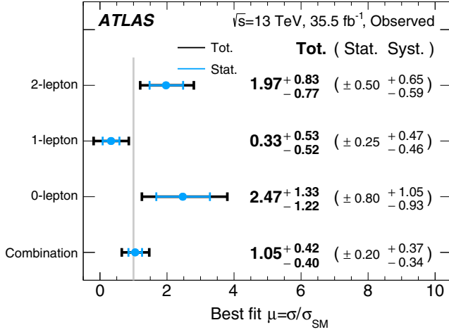
FIG. 7. The fitted values of the signal-strength parameter \mu_{EW VVjj}^{\text{obs}} for the 0-, 1- and 2-lepton channels and their combination. The individual \mu_{EW VVjj}^{\text{obs}} values for the lepton channels are obtained from a simultaneous fit with the signal-strength parameter for each of the lepton channels floating independently. The probability that the signal strengths measured in the three lepton channels are compatible is 36%.
