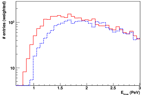
FIG. 5. Distribution of true energy of gamma-ray (red, solid) and proton (blue, dotted) showers for an energy cut E_{\text{reco}} > 1.4 PeV, weighted to a E^{-2.7} spectrum.
