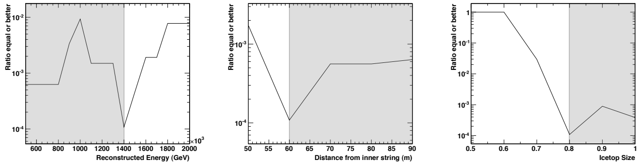
FIG. 6. Optimization scans for cut parameters E_{\min} , d_{\max} , and C_{\max} . The fraction of scrambled data sets that perform equal or better than the real data set is plotted against cut value. For each plot, the other 2 parameters are kept constant at their optimal value. The actual scan was done three dimensionally. For each plot, the shaded region indicates the parameter space that is excluded by the optimized cuts.
