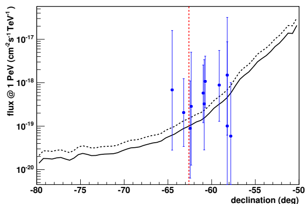
FIG. 15. IceCube 5 year sensitivity to point sources as a function of declination. The solid (dashed) black line indicates the sensitivity to an E^{-2} ( E^{-2.5} ) flux. The dashed red line indicates the lowest declination reached by the Galactic Plane. The blue points indicate the flux at 1 PeV with extrapolated uncertainties of the sources listed in Table I in the absence of a cut-off.
