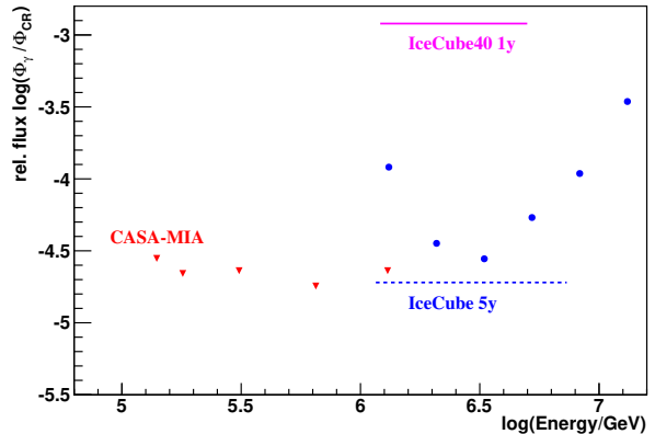
FIG. 14. Existing limits (red triangles for CASA-MIA and purple line for present IC40 analysis) and IceCube sensitivity to a diffuse gamma-ray flux from a region within 10 degrees from the Galactic Plane. The blue dashed line indicates the five year sensitivity of the completed detector, while the blue dots represent the sensitivity in smaller energy bins.
