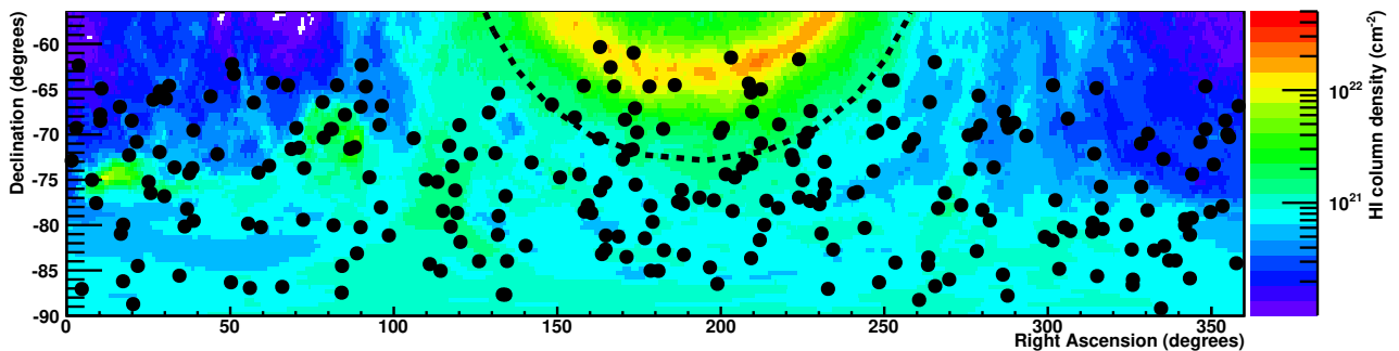
FIG. 7. Equatorial map of the 268 candidate gamma-ray events of the IC40 data set superimposed on HI column densities based on [14]. The dotted black curve encloses the source region, defined as within 10 degrees of the Galactic Plane.
