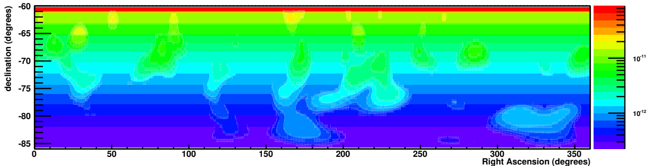
FIG. 10. Sky map of 90% C.L. upper limits on point source flux (E/\text{TeV})^2 d\Phi/dE in \text{cm}^{-2}\text{s}^{-1}\text{TeV}^{-1} for E^{-2} source spectra in the energy range E = 1.2 - 6.0 PeV. The limit is typically more constraining at low declinations where the effective area is largest.
