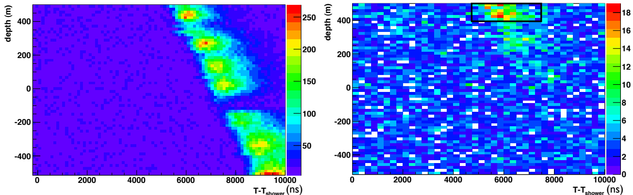
FIG. 11. Observed time of isolated hits (SLC) relative to the arrival time of the air shower front measured by IceTop. The left plot shows the distribution of SLC hits for all events; the right plot is the same but restricted to the subset of events which have only SLC hits and no HLC hits. There is an excess of SLC hits in the region where a muon signal associated to the shower is expected. This allows an additional cut to separate gamma-ray showers from hadronic showers. The black box indicates the region in which an SLC hit counts as a veto (see text for details). The variation in the number of hits as a function of depth in the left plot is due to variations in the optical properties of the ice.
