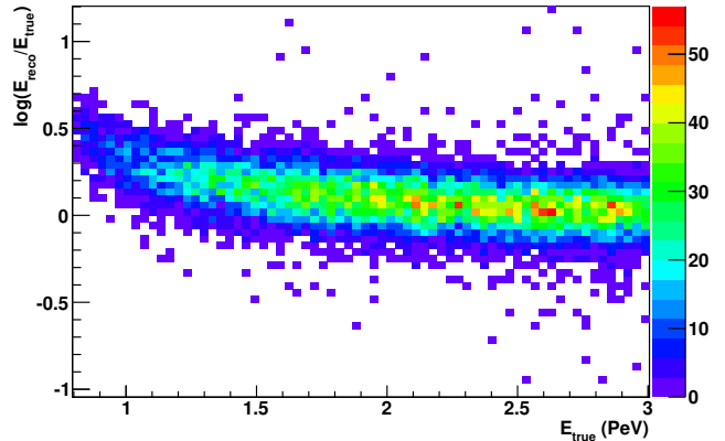
FIG. 4. Ratio between reconstructed and true energy of simulated gamma-ray showers as a function of their true energy. At low energies the overestimation of the gamma-ray energy is largely due to a bias effect of the eight-station filter. At higher energies, this overestimation decreases.
