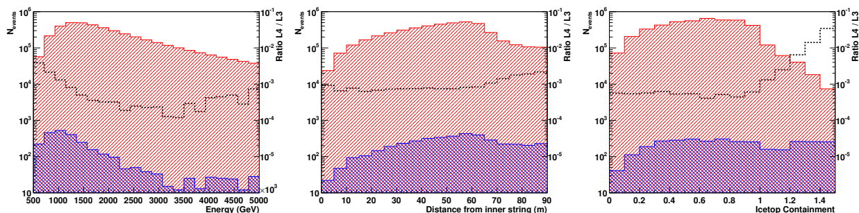
FIG. 12. The number of L3 (red) and L4 (blue) events in the data as a function of the three main cut parameters. The ratio of the number of L4 to L3 events is given by the black dotted line, for which the corresponding axis is drawn on the right-hand side of the plot.
