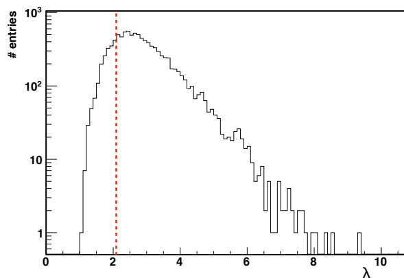
FIG. 9. Distribution of the largest value of \lambda observed in each scrambled data set. The red dotted line indicated the value for \lambda that corresponds to the hottest spot in the data.
