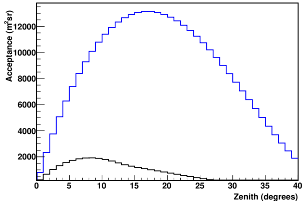
FIG. 13. Acceptance (effective area integrated over solid angle) for showers with an axis through both IceTop and IceCube for IC40, C_{IT}=0.8 (black), and IC86, C_{IT}=1.0 (blue).
