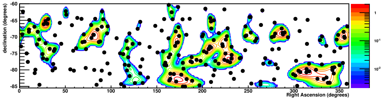
FIG. 8. Equatorial map of the part of the sky for which an unbinned point source search is performed. The contours indicate the value of \lambda and the black dots are the candidate events.
