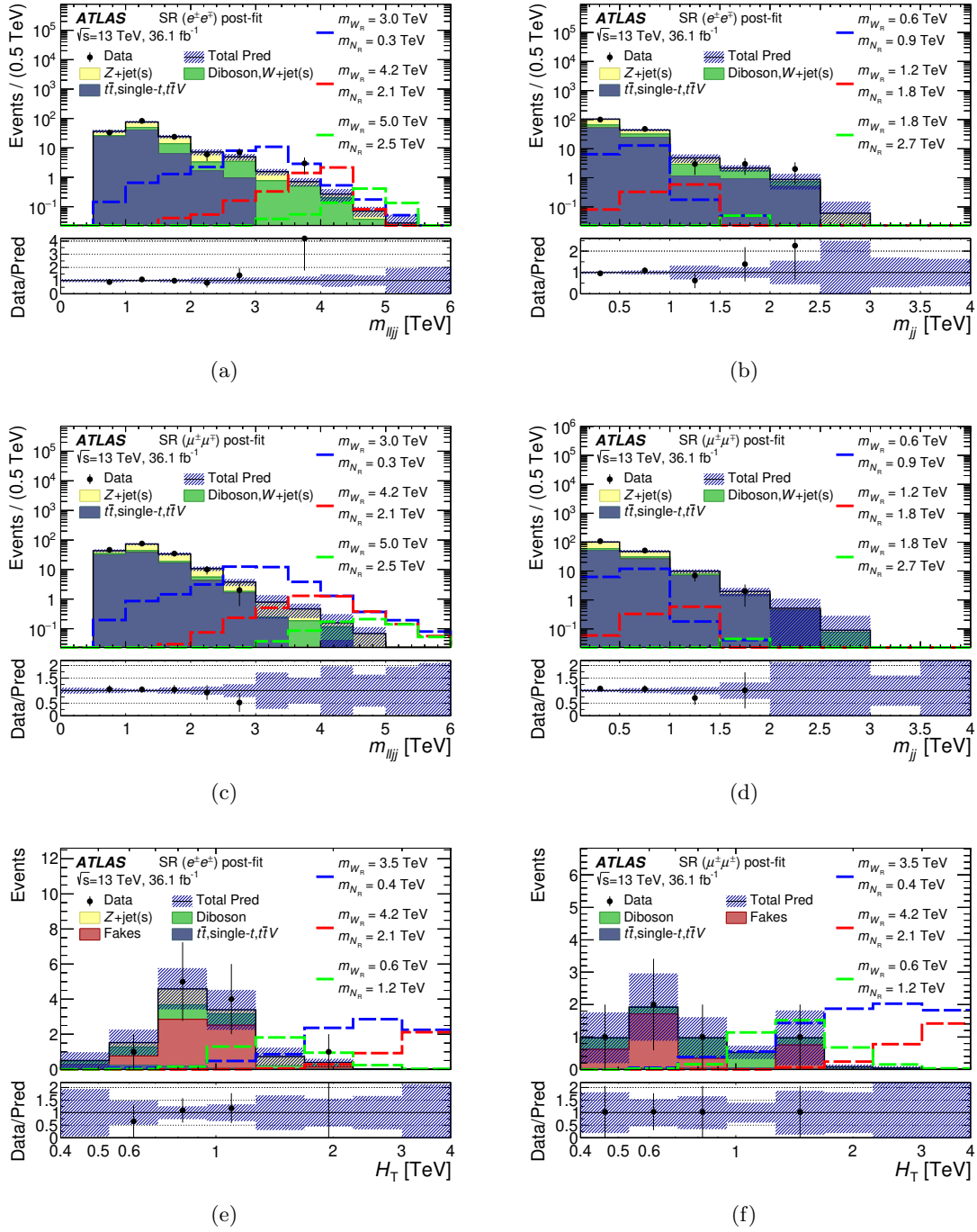
Figure 6. Distributions for data and background predictions after the CR+SR fit for discriminant variables in various signal regions and channels: (a) m_{\ell\ell jj} in SR( e^\pm e^\mp ), (b) m_{jj} in SR( e^\pm e^\mp ), (c) m_{\ell\ell jj} in SR( \mu^\pm \mu^\mp ), (d) m_{jj} in SR( \mu^\pm \mu^\mp ), (e) H_T in SR( e^\pm e^\pm ), and (f) H_T in SR( \mu^\pm \mu^\pm ). The hatched bands include all post-fit systematic uncertainties. The correlation between sources of systematic uncertainties are taken into account. A few simulated signal distributions, normalised to the predicted cross-section, are overlaid on top of the background prediction in the plots. The last bin in each histogram contains the overflow.
