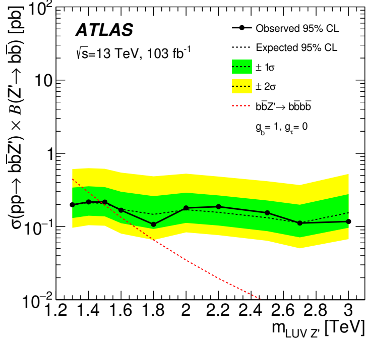
Figure 4: The observed (solid) and expected (dashed) 95% CL upper limits on the production of Z' \rightarrow b\bar{b} in association with b -quarks. The bands surrounding the expected limit show the 68% and 95% confidence intervals. The predicted cross sections of the LUV Z' model with g_b set to unity and g_\tau set to zero, calculated at LO with MADGRAPH5_aMC@NLO, are also overlaid.
