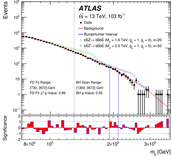
Figure 3: Background estimate from the FD method with N = 3 and data in the SR. The solid squares show the dijet invariant mass spectrum in data and the solid curve is the background estimated by the FD method. The BumpHunter algorithm scans the mass region above 1.3 TeV as indicated by the vertical dashed line. The vertical solid lines refer to the boundaries of the most significant interval flagged by BumpHunter ; this is found to be [1921, 2114] GeV for which the p -value is stated in the figure. Open squares (circles) are the signal distributions of the 1.6 (2.5) TeV LUV Z' boson on top of the data with the cross sections inflated by a factor of 20 (50). The lower panel shows the significance calculated using the background estimate and data. The significance is defined as (d_i - b_i)/\delta , where d_i refers to the data count while b_i refers to the background estimate, and \delta is an uncertainty taking both the uncertainty on the data count and background estimate into account [57].
