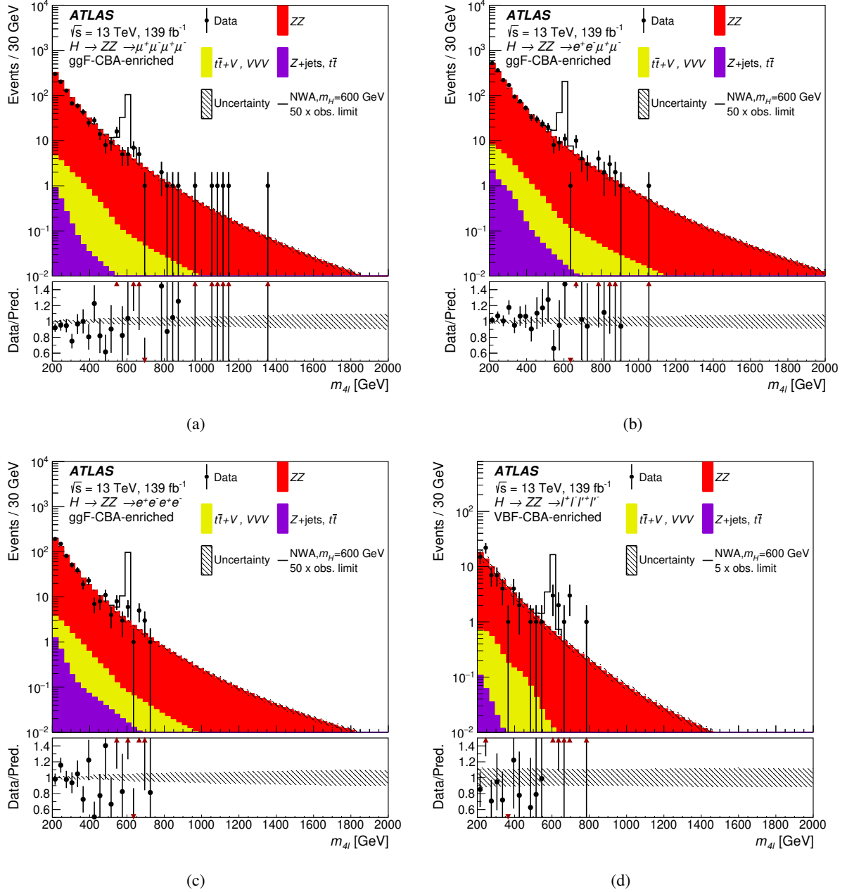
Figure 9: Distribution of the four-lepton invariant mass m_{4\ell} in the \ell^+ \ell^- \ell'^+ \ell'^- search for (a),(b),(c) the ggF-CBA-enriched categories and (d) the VBF-CBA-enriched category. The backgrounds are determined from a combined likelihood fit to the data under the background-only hypothesis. The simulated m_H = 600 GeV signal is normalised to a cross section corresponding to 50 (5) times the observed limit given in Section 9.1.1 for the ggF (VBF) production mode. The error bars on the data points indicate the statistical uncertainty, while the systematic uncertainty in the prediction is shown by the hatched band. The lower panels show the ratio of data to prediction.
