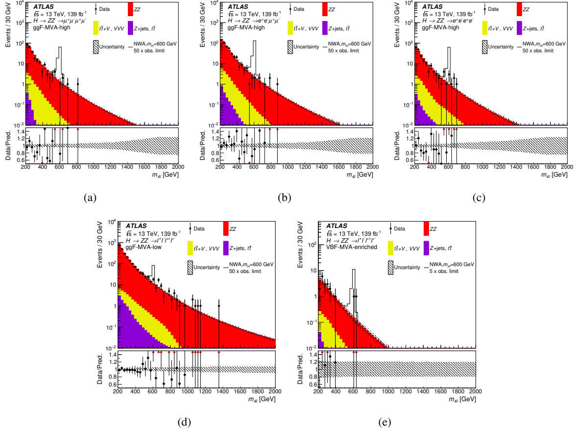
Figure 2: Distributions of the four-lepton invariant mass m_{4\ell} in the \ell^+\ell^-\ell^+\ell^- search for the ggF-MVA-high categories ( \mu^+\mu^-\mu^+\mu^- (a), e^+e^-\mu^+\mu^- (b), and e^+e^-e^+e^- (c) final states), for the ggF-MVA-low category (d), and for the VBF-MVA-enriched category (e). The backgrounds are determined from a combined likelihood fit to the data under the background-only hypothesis. The simulated m_H = 600 GeV signal is normalised to a cross section corresponding to 50 (5) times the observed limit given in Section 9.1.1 for the ggF (VBF) production mode. The error bars on the data points indicate the statistical uncertainty, while the systematic uncertainty in the prediction is shown by the hatched band. The lower panels show the ratio of data to prediction. The red arrows indicate data points that are outside the displayed range.
