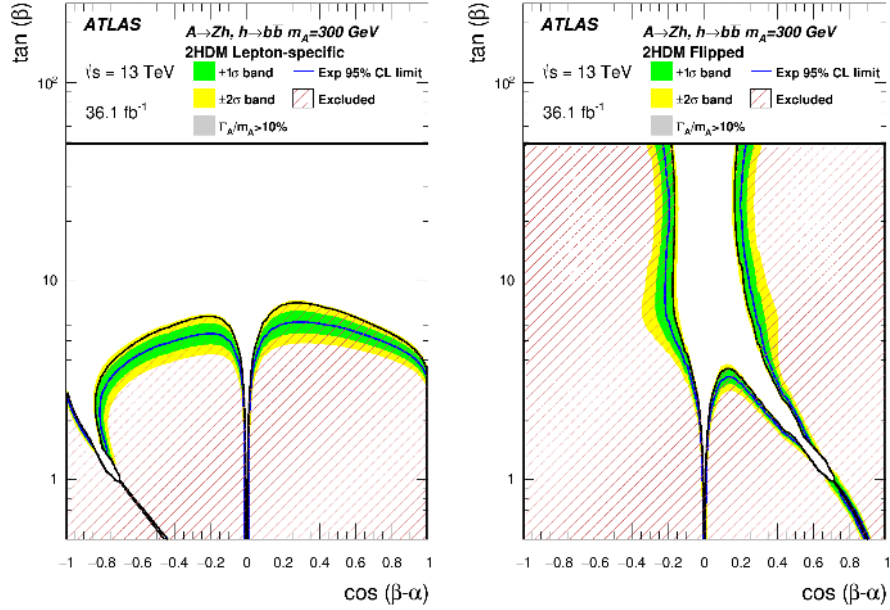
(c) 2HDM Lepton-specific
