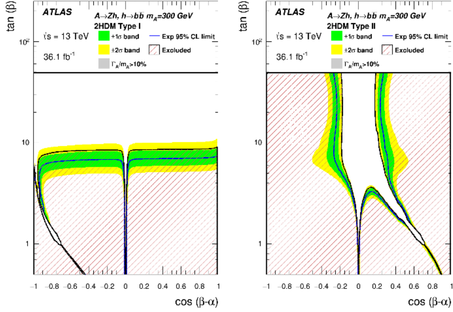
(a) 2HDM Type-I
