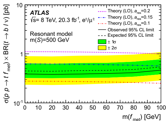
Fig. 6 Observed and expected limits on the cross section times branching ratio ( left ) for the resonant model with m(S) = 500 \text{ GeV} and ( right ) for the non-resonant model, as a function of the mass of f_{\text{met}} and v_{\text{met}} ,
