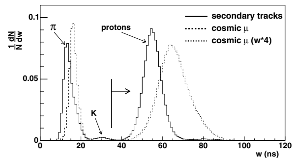
FIG. 1. The distribution of the COT dE/dx variable w for positively charged secondary [19] tracks in the momentum range of 300–350 MeV/ c (solid line), for high- p_T cosmic-ray muons (dashed line), and the expectation for H^{\pm\pm} tracks (dotted line). The latter is modeled by quadrupling the w measurements of cosmic-ray muons. The arrow indicates the signal selection region.
