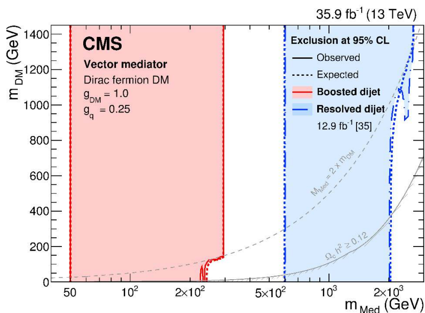
Figure 8. The 95% CL observed (solid red) and expected (dashed red) excluded regions in the plane of dark matter particle mass ( m_{DM} ) vs. mediator mass ( m_{Med} ), for vector mediators. A branching fraction of 100% is assumed for a leptophobic vector mediator decaying to dijets. The exclusion is computed for a quark coupling choice g_q = 0.25 and for a dark matter coupling g_{DM} = 1 . The excluded regions from the dijet resolved analysis (blue dot dashed lines) using early 2016 data [35] are also shown. Results are compared to constraints from the cosmological relic density of DM (light gray) determined from astrophysical measurements [74, 75] and MADDM version 2.0.6 [76, 77] as described in ref. [78].
