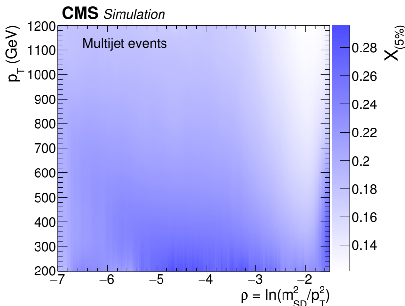
Figure 2. The distribution of X_{(5\%)} used to define the N_2^{1,\text{DDT}} variable, corresponding to the 5% quantile of the N_2^1 distribution in simulated multijet events. The distribution is shown as a function of the jet \rho and p_T and smoothed using a kNN approach [64]. The N_2^1 distribution is mostly insensitive to the jet \rho and p_T in the kinematic phase space considered for this analysis ( -5.5 < \rho < -2.0 ). Residual correlations in simulation are corrected by applying a decorrelation procedure that yields the N_2^{1,\text{DDT}} variable.
