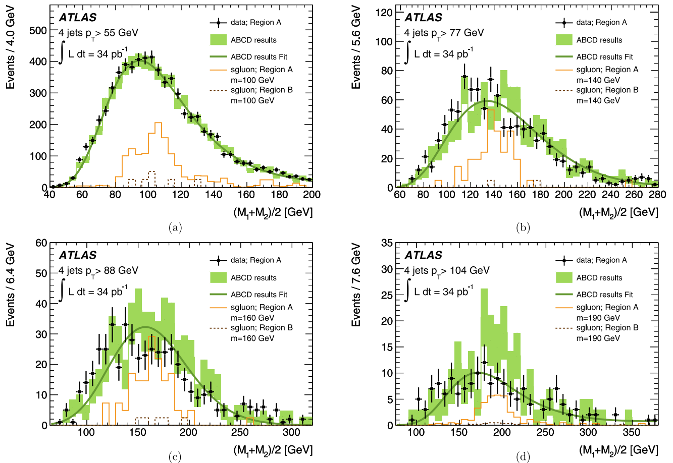
Fig. 2 The comparison of the prediction of the background with the data in the signal region is shown. The points are the data in the signal region (region A). The solid (dashed) histogram is the estimated signal in region A (B) for the nominal cross section. The predictions of background in region A based upon the data in region B (rectangles) and
