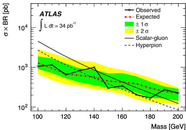
Fig. 3 Expected and observed 95% CL upper bounds on the product of the scalar pair production cross sections and of the branching ratio to gluons as a function of the scalar mass. The predictions of the sgluon and hyperpion pair production cross section are also shown
