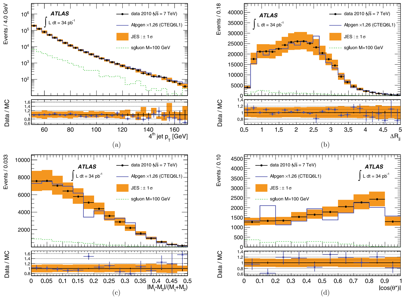
Fig. 1 Kinematic variables at different stages of the analysis. Data (dots) are compared to the ALPGEN MC sample (solid line). The solid band corresponds to one standard deviation in the jet energy scale. The ratio data/MC is also shown with its statistical uncertainty, which is dominated by the MC statistics. The dashed line corresponds to a sgluon signal of 100 GeV. (a) The transverse momentum of the 4th jet is shown. (b) The \Delta R_{jj} distribution for the reconstructed sgluon candidate with the highest transverse momentum jet is shown after requiring the transverse momentum to be greater than 55 GeV and pairing the four leading jets into two sgluon candidates. (c) The relative mass difference is shown after the criterias on the p_T and \Delta R_{jj} have been applied. (d) The scattering angle in the 4-jet center-of-mass frame is shown after all other selection criteria have been applied
