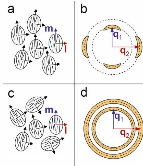
FIG. 4. Orientation of the transverse molecular directors \mathbf{m} , \mathbf{l} in N_b with \mathbf{n} perpendicular to the drawing: transverse directors aligned by (a) an external field or (c) randomly distributed in the plane orthogonal to \mathbf{n} . The ellipses represent micron-sized domains (each one consisting of uniformly aligned nanometer-sized cybotactic clusters) where the orientation of the molecular director is spontaneously uniform. (b) and (d) show the corresponding WA diffraction patterns. The latter would be indistinguishable from that of a composite N_u comprised of randomly oriented nano-sized biaxial clusters.
