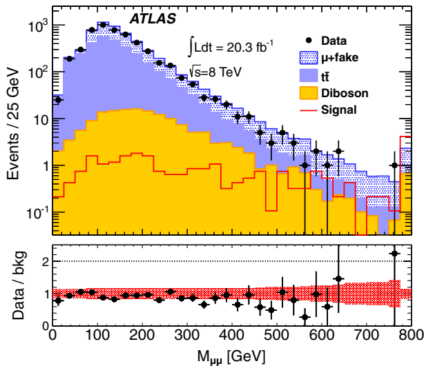
FIG. 2 (color online). The dimuon invariant mass ( M_{\mu\mu} ) distribution for the predicted background and observed data for like-sign dimuon events where the leading muon satisfies p_T > 100 GeV. The background histograms are stacked. The signal histogram is overlaid. The last bin along the x axis shows the overflows. The bottom panel shows the ratio of data to the expected background (points) and the total uncertainty on the background (shaded area).
