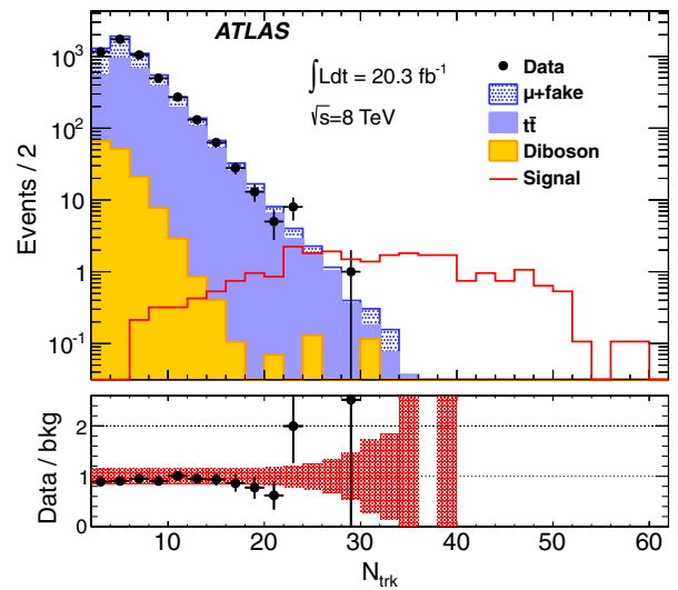
FIG. 4 (color online). The track multiplicity ( N_{\text{trk}} ) distribution ( p_T^{\text{trk}} > 10 GeV) for the predicted background and observed data for events where the leading muon has p_T > 100 GeV. The background histograms are stacked. The signal histogram is overlaid. The bottom panel shows the ratio of data to the expected background (points) and the total uncertainty on the background (shaded area).
