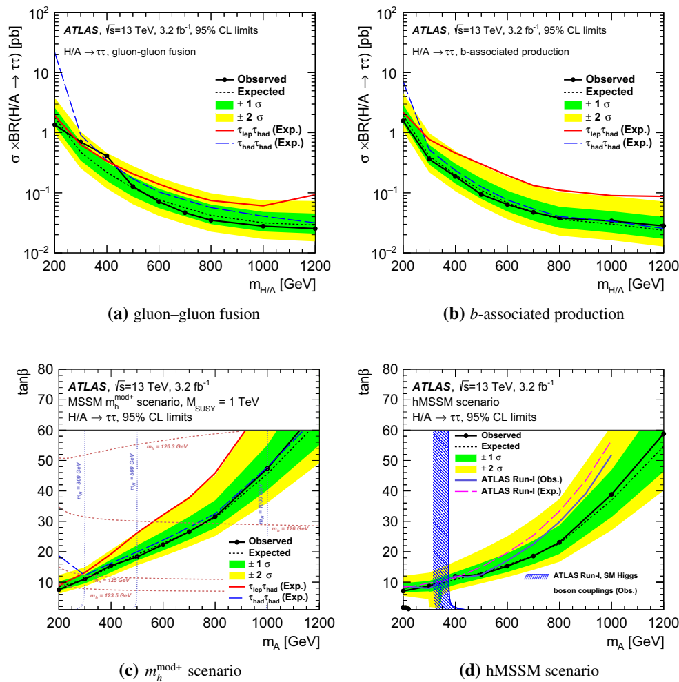
Fig. 5 The observed and expected 95% CL upper limits on the production cross section times branching fraction of a scalar particle decaying to a pair of \tau leptons is performed using a data sample corresponding to an integrated luminosity of 3.2 \text{ fb}^{-1} from proton–proton collisions at \sqrt{s} = 13 \text{ TeV} recorded by the ATLAS detector at the LHC. The search finds no indication of an excess over the expected background in the channels considered. Limits are set at the 95% CL, which provide constraints in the MSSM parameter space. Model-independent upper limits on the production cross section times the \tau\tau branching fraction of a scalar boson versus its mass, in both the gluon–gluon fusion and b -associated production modes, are presented. The upper limits on the cross
