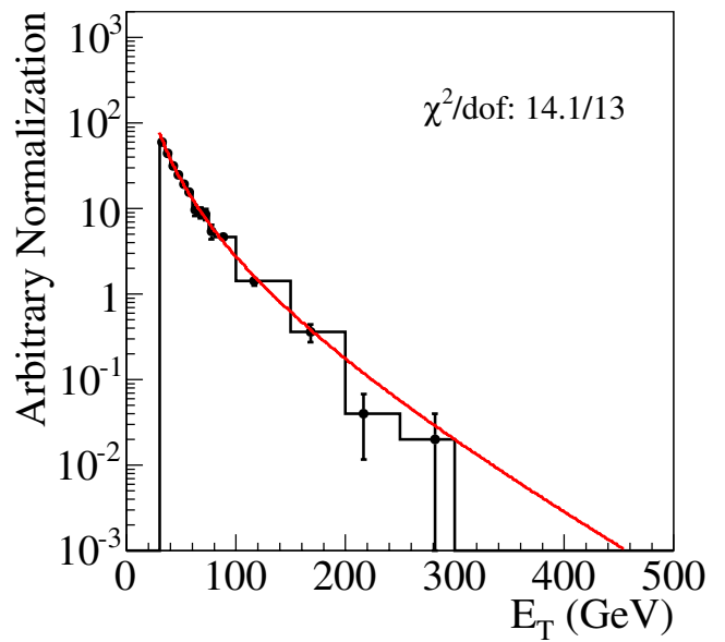
FIG. 32 (color online). E_T distribution of jets in N_{\text{jet}}^{30} = 2 Z \rightarrow ee and Z \rightarrow \mu\mu events. The distribution is fit to Eq. (1) in the E_T > 30 GeV region with the parameter p_2 fixed to that obtained from the fit in Fig. 31.
