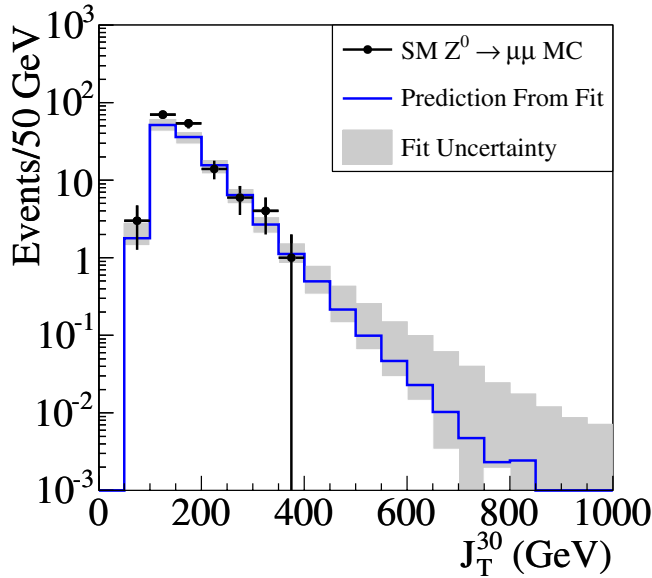
FIG. 11 (color online). The prediction for the J_T^{30} distribution (blue, solid line) of standard model Z Monte Carlo and its uncertainty (gray band), compared to the actual distribution (black points with errors).
