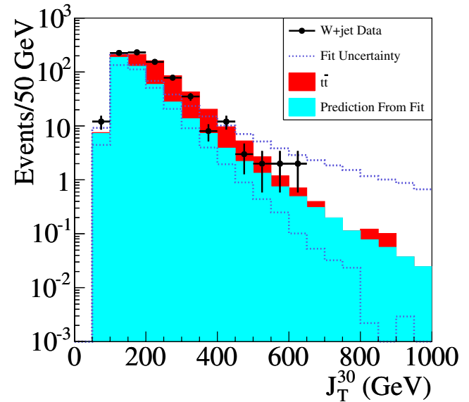
FIG. 27 (color online). The prediction (cyan, light shaded histogram) and uncertainty (dotted lines) for the J_T^{30} distribution of W + jet events. The expectation from t\bar{t} is added to the prediction. The data (points with errors) agree with the background plus t\bar{t} hypothesis.
