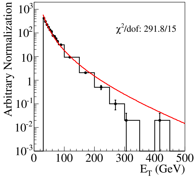
FIG. 24 (color online). E_T distribution of jets in N_{\text{jet}}^{30} = 2 W + jet events. The distribution is fit to Eq. (1) in the E_T > 30 GeV region with the parameter p_2 fixed to that obtained from the fit in Fig. 23.
