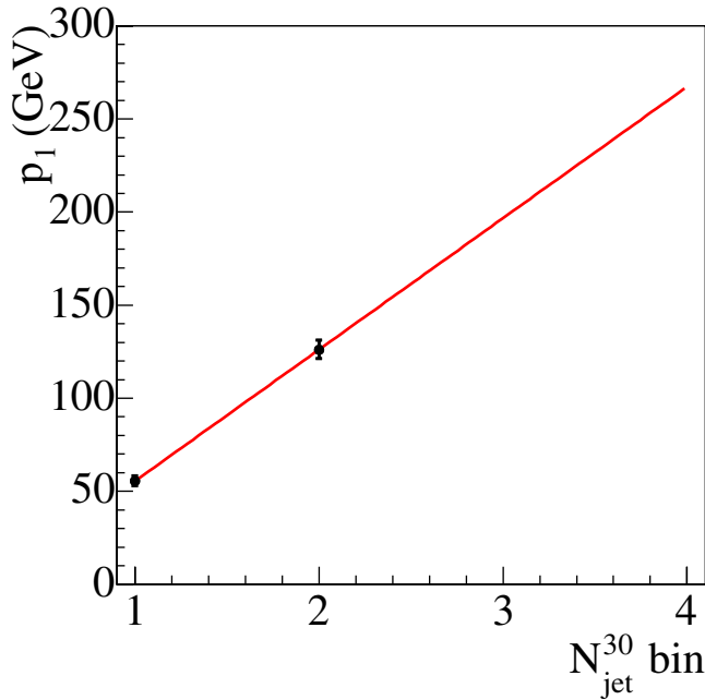
FIG. 25 (color online). The extrapolation of the exponential parameter p_1 vs N_{\text{jet}}^{30} in W + jet events.
