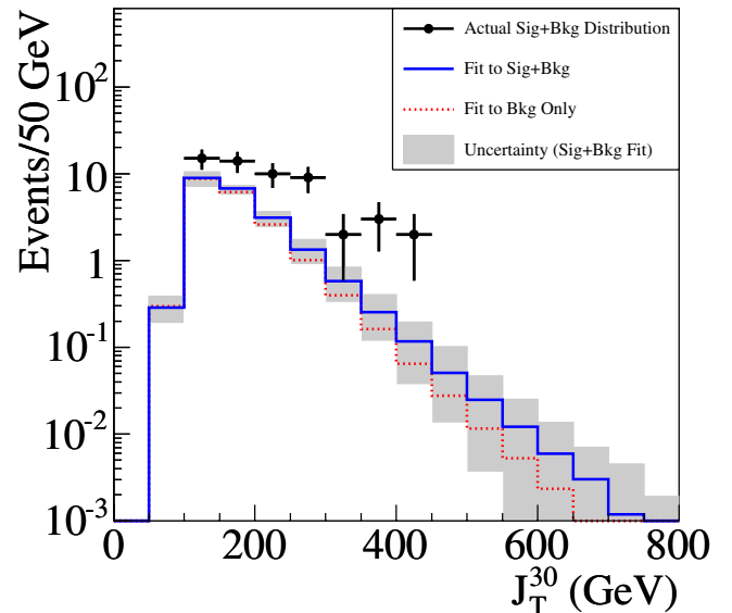
FIG. 29 (color online). Prediction for the J_T^{30} distribution in standard model Z \rightarrow \mu\mu events, with and without the presence of a 200 \text{ GeV}/c^2 b' signal introduced. The difference between the two predictions is small compared to the excess of signal at large J_T^{30} .
