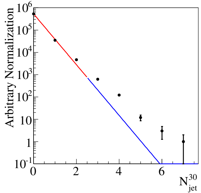
FIG. 26 (color online). N_{\text{jet}}^{30} distribution in W + jet events. The distribution is fit to an exponential in the range N_{\text{jet}}^{30} \leq 2 .
