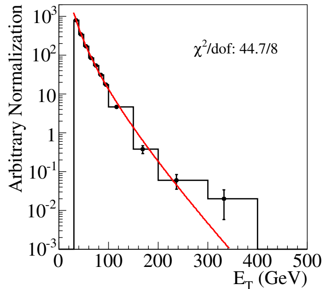
FIG. 13 (color online). E_T distribution of jets in N_{\text{jet}}^{30} = 1 “X” + jet events, selected with the jet triggers as described in the text. The distribution is fit to Eq. (1) in the E_T > 30 GeV region.
