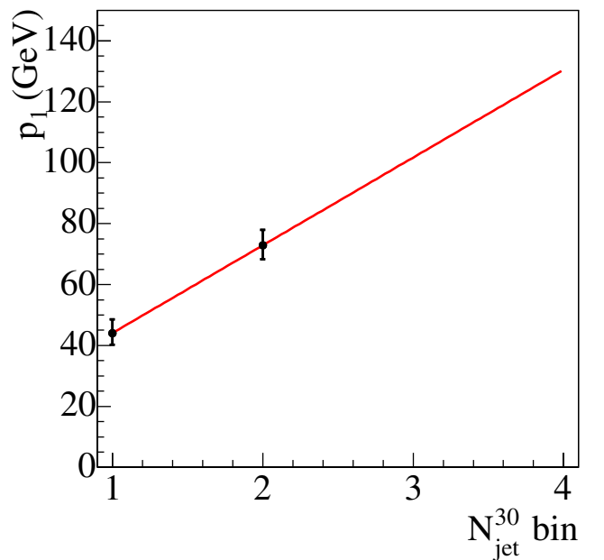
FIG. 33 (color online). The extrapolation of the exponential parameter p_1 vs N_{\text{jet}}^{30} in Z \rightarrow ee and Z \rightarrow \mu\mu events.
