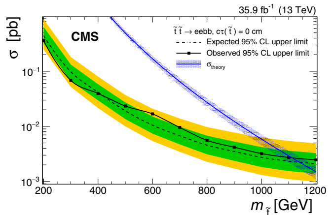
FIG. 10. Expected and observed upper limits at 95% C.L. on the RPV SUSY \tilde{t}\tilde{t} squark pair production cross section as a function of M_{\tilde{t}} for c\tau = 0 cm. The expected limits represent the median values, while the inner green and outer yellow bands are the 68% and 95% confidence intervals, respectively.
