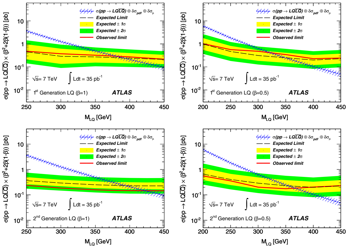
FIG. 5 (color online). 95% CL upper bounds on the LQ pair production cross sections as a function of LQ mass for the combination of the eejj and the evjj channels (top), and for the \mu\nu jj and the \mu\mu jj channels (bottom). The figures on the left (right) show the limit for \beta = 1.0 ( 0.5 ). The expected limit is indicated by the dashed line. The light yellow (dark green) solid band contains 68% (95%) of possible outcomes from pseudoexperiments in which the yield is Poisson fluctuated around the background-only expectation. Systematic uncertainties are included. The observed limit is indicated by the solid line. The theory prediction is indicated by the dotted line, which includes systematic uncertainties due to the choice of the PDF and to the renormalization and factorization scales ( \Delta\sigma_\mu ).
