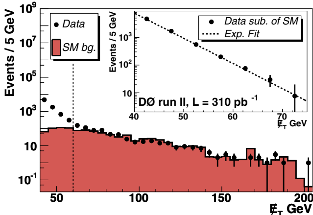
FIG. 1 (color online). Distribution in \cancel{E}_T after applying all criteria, except \cancel{E}_T > 60 GeV (C1). The dark shaded area corresponds to the SM simulation. A fit by an exponential to \cancel{E}_T < 60 GeV, after subtraction of the contributions from the SM, shown in the figure insert, is used to estimate the instrumental background.
