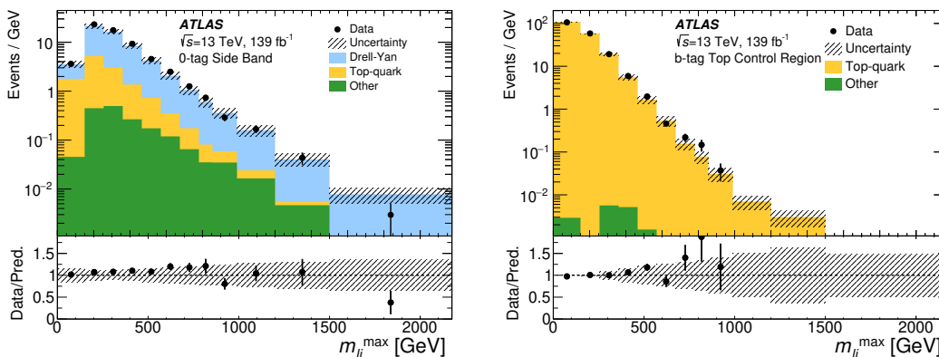
Figure 2. Distributions of m_{\ell j}^{\max} in the combined be and b\mu 0-tag SB for the bl channels (left) and the b -tag Top CR for the cl channels (right). The total modelling uncertainty combined with the MC statistical error is shown as the hatched band as explained in section 7. The category ‘Other’ represents the sum of all SM background contributions except those from top-quark processes ( t\bar{t} and single-top) and, for the 0-tag SB distribution, Drell-Yan processes.
