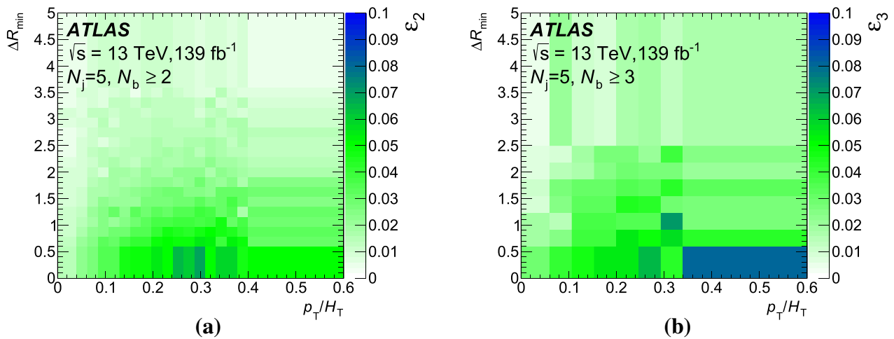
Fig. 3 Two-dimensional distributions of the probability a \epsilon_2 or b \epsilon_3 of b -tagging an additional jet in a sample of events with a at least two or b at least three b -tagged jets as a function of the ratio of jet transverse momentum to H_T , p_T/H_T , and the minimum \Delta R between the jet and
