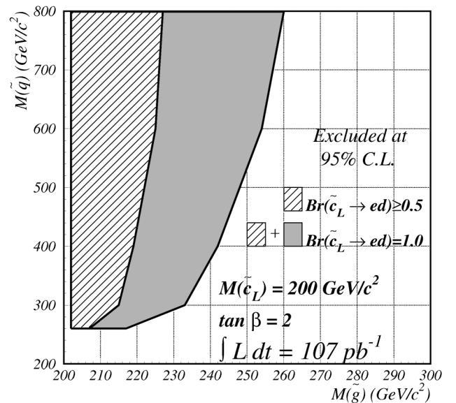
FIG. 2. Exclusion region in the \tilde{g} - \tilde{q} mass plane for the charm squark analysis. The branching ratio to LS ee is calculated using the scenario in Ref. [7], which requires M(\tilde{g}) > M(\tilde{c}_L) .
