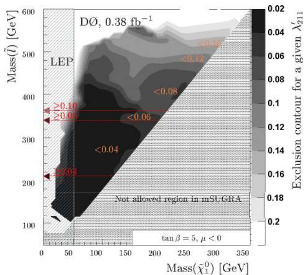
FIG. 3: 95% C.L. exclusion contour on \lambda_{211}^2 couplings within the mSUGRA framework for \tan \beta = 5 and \mu < 0 . The arrows indicate limits on the slepton mass \tilde{l} , for a given coupling \lambda_{211}^2 .
