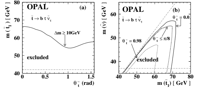
Fig. 10. The 95% C.L. excluded regions assuming that \tilde{t}_1 always decays into b\tau\tilde{\nu} . a The excluded regions in the (\theta_{\tilde{t}_1}, m_{\tilde{t}_1}) plane where the mass difference between the \tilde{t}_1 and the \tilde{\nu} is greater than 10 GeV. The dash-dotted straight line shows the kinematic limit for this decay, since a \tilde{\nu} lighter than 37.1 GeV has been excluded [9, 10]. b The excluded regions in the (m_{\tilde{t}_1}, m_{\tilde{\nu}}) plane, for a mixing angle of the \tilde{t}_1 assumed to be 0.0 (solid line), smaller than \pi/8 rad (dashed line), and 0.98 rad (dotted line). The dash-dotted horizontal line shows the limit on m_{\tilde{\nu}} obtained at LEP1, and the dash-dotted diagonal line shows the kinematic limit for the \tilde{t}_1 \rightarrow b\tau\tilde{\nu} decay
