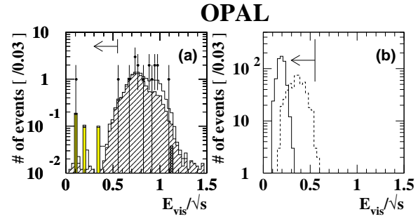
Fig. 6. The distributions of the visible energy normalised to the centre-of-mass energy after cut (B3) for background ( histograms ) and data in a , and for the \tilde{\tau}_1\tilde{\tau}_1 signal predictions in b . The conventions for the various histograms are the same as in Fig. 5
