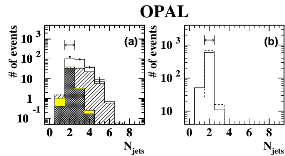
Fig. 2. The distributions of the number of reconstructed jets after all preselections: for background ( histograms ) and data in a , and for \tilde{\tau}_1\tilde{\tau}_1 predictions in b . The conventions for the various histograms are the same as in Fig. 1
