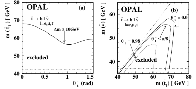
Fig. 9. The 95% C.L. excluded regions assuming that the \tilde{t}_1 decays into b\ell\tilde{\nu} and that the branching fraction to each lepton flavour is the same. a The excluded regions in the (\theta_{\tilde{t}_1}, m_{\tilde{t}_1}) plane where the mass difference between the \tilde{t}_1 and the \tilde{\nu} is greater than 10 GeV. The dash-dotted straight line shows the kinematic limit for this decay, since a \tilde{\nu} lighter than 37.1 GeV has been excluded [9, 10]. b The excluded regions in the (m_{\tilde{t}_1}, m_{\tilde{\nu}}) plane, for a mixing angle of the \tilde{t}_1 assumed to be 0.0 (solid line), smaller than \pi/8 rad (dashed line), and 0.98 rad (dotted line). The dash-dotted horizontal line shows the limit on m_{\tilde{\nu}} obtained at LEP1, and the dash-dotted diagonal line shows the kinematic limit for the \tilde{t}_1 \rightarrow b\ell\tilde{\nu} decay
