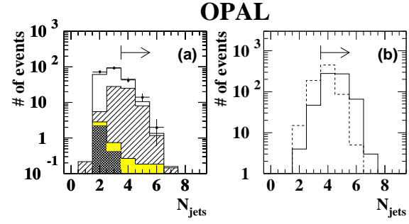
Fig. 5. The distributions of the number of reconstructed jets after cut (B1). The arrows in these figures show the selection criteria. a shows the distribution of the data with error bars. The predictions from background processes are also shown: dilepton events ( cross hatched area ), two-photon processes ( grey area ), four-fermion processes ( singly hatched area ), and the multi-hadronic events ( open area ). b shows predictions for \tilde{\tau}_1\tilde{\tau}_1 in which \tilde{\tau}_1 decays into b\ell\tilde{\nu} . The continuous line histogram is for (m_{\tilde{\tau}_1}, m_{\tilde{\nu}}) = (70 \text{ GeV}, 55 \text{ GeV}) , and the dotted line is for (70 \text{ GeV}, 35 \text{ GeV}) . In these samples, the branching fraction to each lepton flavour is assumed to be the same
