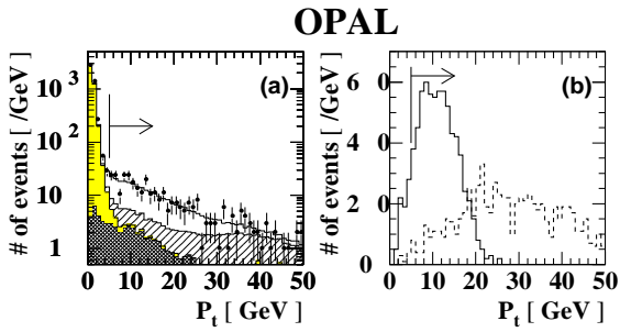
Fig. 1. The distributions of P_t after cut (P3) for background ( histograms ) and data in a , and for \tilde{\tau}_1\tilde{\tau}_1 predictions in b . The arrows in these figures show the selection criteria. In a the distribution of the data is shown by the points with error bars . The predictions from background processes are also shown: dilepton events ( cross hatched area ), two-photon processes ( grey area ), four-fermion processes ( singly hatched area ), and multihadronic events ( open area ). b shows predictions for \tilde{\tau}_1\tilde{\tau}_1 in which \tilde{\tau}_1 decays into c\tilde{\chi}_1^0 . The continuous line histogram is for (m_{\tilde{\tau}_1}, m_{\tilde{\chi}_1^0})=(70\text{ GeV}, 60\text{ GeV}) , and the dashed line is for (70\text{ GeV}, 35\text{ GeV}) , starting from 1000 generated events for each
