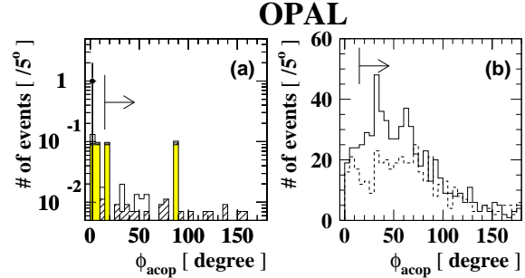
Fig. 7. The distributions of the acoplanarity angle after cut (B5) for background ( histograms ) and data in a , and for the \tilde{\tau}_1\tilde{\tau}_1 predictions in b . The conventions for the various histograms are the same as in Fig. 5
