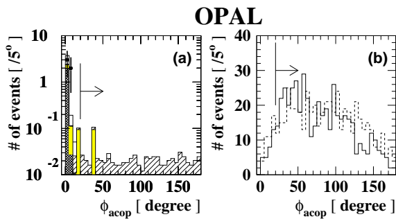
Fig. 4. The distributions of the acoplanarity angle after cut (A3) for background (histograms) and data in a , and for the \tilde{t}_1\tilde{t}_1 predictions in b . The conventions for the various histograms are the same as in Fig. 1
