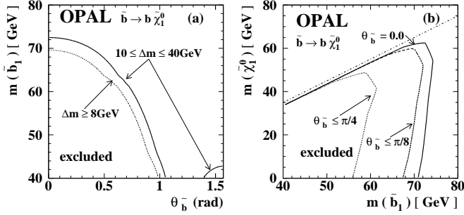
Fig. 11. The 95% C.L. excluded regions assuming that the \tilde{b}_1 decays into b\tilde{\chi}_1^0 . a The excluded region in the (\theta_{\tilde{b}_1}, m_{\tilde{b}_1}) plane for a mass difference, \Delta m (= m_{\tilde{b}_1} - m_{\tilde{\chi}_1^0}) , 10 \leq \Delta m \leq 40 GeV. The dotted line shows the excluded region for \Delta m \geq 8 GeV. b The excluded regions in the (m_{\tilde{b}_1}, m_{\tilde{\chi}_1^0}) plane, for a mixing angle of the \tilde{b}_1 assumed to be 0.0 (solid line), smaller than \pi/8 rad (dashed line), and smaller than \pi/4 (dotted line). The dash-dotted line shows the kinematic limit for the \tilde{b}_1 \rightarrow b\tilde{\chi}_1^0 decay
