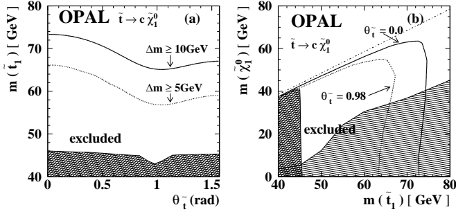
Fig. 8. The 95% C.L. excluded regions assuming that the \tilde{t}_1 decays into c\tilde{\chi}_1^0 . a The excluded regions in the (\theta_{\tilde{t}_1}, m_{\tilde{t}_1}) plane. The solid line shows the limit for a mass difference \Delta m (= m_{\tilde{t}_1} - m_{\tilde{\chi}_1^0}) \geq 10 GeV, and the dotted line for \Delta m \geq 5 GeV. The cross hatched region has already been excluded by the search at LEP1 [6]. b The excluded regions in the (m_{\tilde{t}_1}, m_{\tilde{\chi}_1^0}) plane, for a mixing angle of \tilde{t}_1 of 0.0 (solid line) and 0.98 rad (dotted line). The cross hatched region has already been excluded by the search at LEP1 [6]. The singly hatched region has been excluded by the D0 Collaboration [5]. The dash-dotted straight line shows the kinematic limit for the \tilde{t}_1 \rightarrow c\tilde{\chi}_1^0 decay
