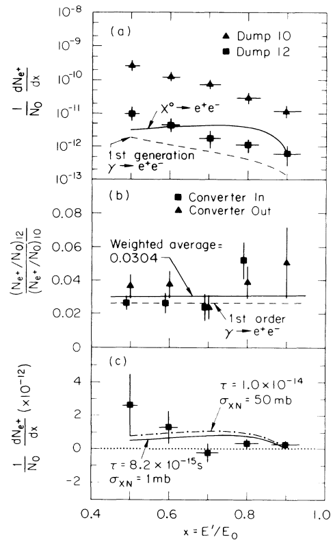
FIG. 1. (a) Number of positrons observed in our angular acceptance divided by the flux of electrons on dump, plotted vs x . Error bars represent statistical and systematic errors added linearly. The solid curve is the e^+ yield expected for dump 12 from a 1.8-MeV axion with \tau = 1 \times 10^{-14} s; the dashed curve represents the corresponding e^+ background from first-generation \gamma punchthrough. (b) Measured ratio of e^+ yields from the two dumps, normalized by respective fluxes of incident electrons; errors shown are dominated by counting statistics. The dashed curve represents the ratio expected from \gamma punchthrough and pair conversion. (c) Residual e^+ yield behind dump 12 after subtraction of 1/27 of the dump-10 yield, compared with net yields expected for a 1.8-MeV axion with lifetimes and absorption cross sections listed.
