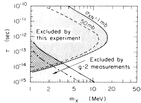
FIG. 2. Regions of m_X and \tau , for a light pseudoscalar boson X^0 decaying predominantly to e^+e^- , that are excluded by this experiment, assuming an absorption cross section of \sigma_{XN} = 1 and 50 mb per nucleon. Also shown are regions excluded by electron g-2 measurements by use of two assumptions (see Refs. 14 and 15) for the possible discrepancy between theory and experiment.
