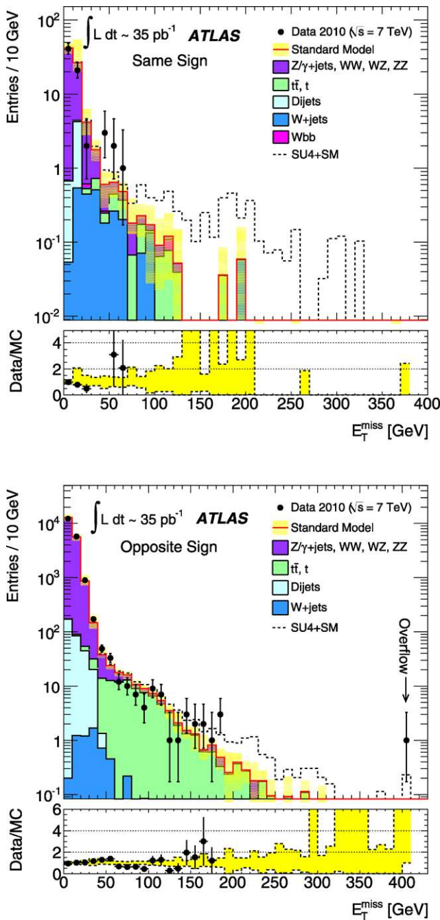
Fig. 1 (Color online) Distributions of E_T^{\text{miss}} for SS ( upper ) and OS ( lower ) lepton pair events passing the analysis selections. The data are shown as points with error bars superimposed on the expected SM background distributions determined (mostly data-driven) with MC simulation. The overflow point in the OS E_T^{\text{miss}} histogram is a likely candidate for cosmic ray interaction. In the bottom panel the ratio between the data and the total SM background is shown. The histogram labelled “Standard Model” represents the sum of all backgrounds and the light ( yellow ) bands indicate the uncertainty on the MC predictions from finite MC statistics and uncertainties in cross section, luminosity and jet and lepton energy scales and resolutions. “SU4” represents a point in the mSUGRA/CMSSM parameter space with m_0 = 200 GeV, m_{1/2} = 160 GeV, A_0 = -400 GeV, \tan \beta = 10 and \mu > 0
