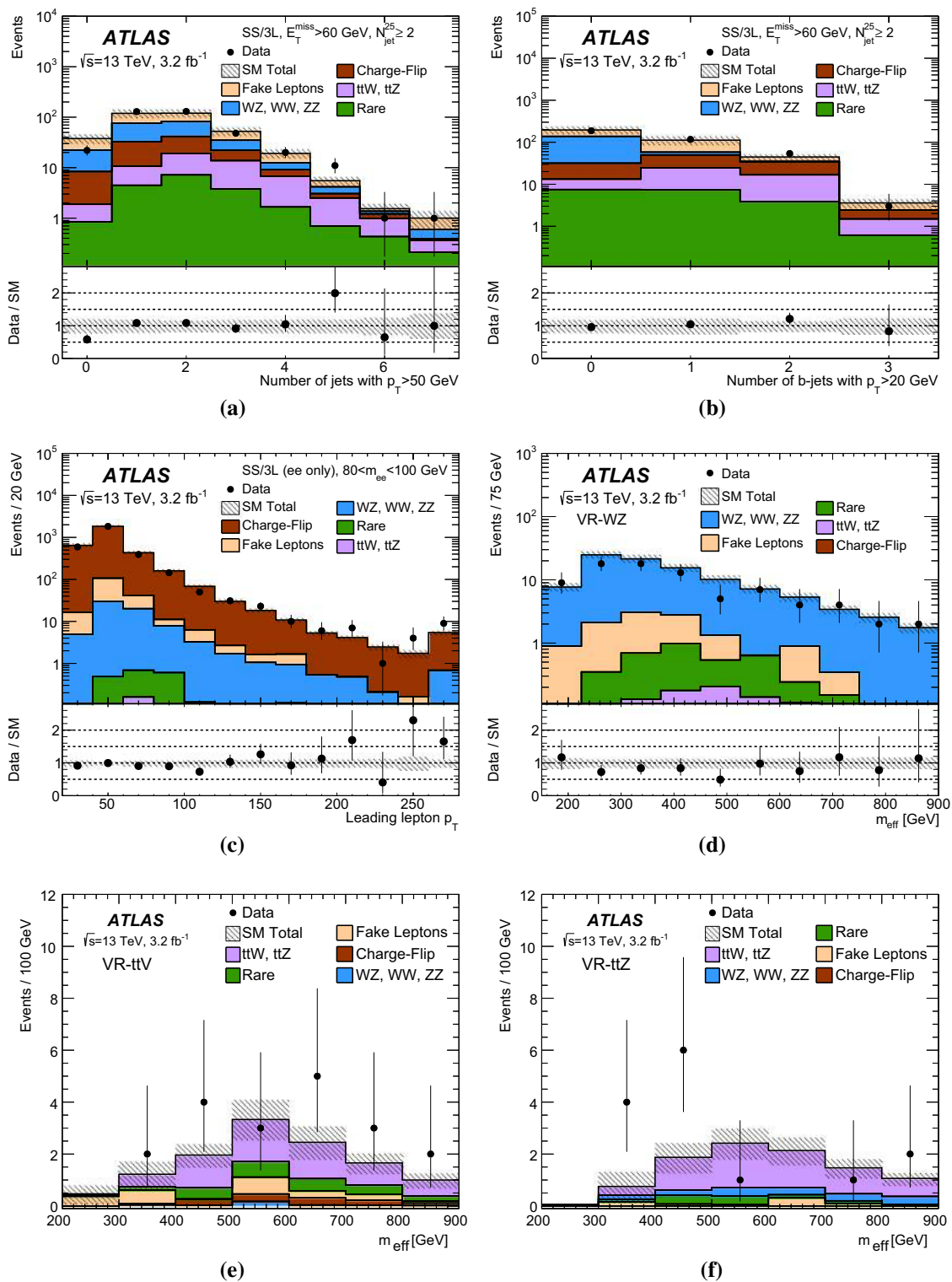
Fig. 2 Distributions of kinematic variables after a SS/3L selection including a, b E_T^{miss} > 60 \text{ GeV} and N_{jet}^{25} \geq 2 , c a b -jet veto and 80 < m_{\ell\ell} < 100 \text{ GeV} , and d-f distributions in the validation regions. The statistical uncertainties in the background prediction are included in the uncertainty band, as well as the theory uncertainties for the backgrounds with prompt SS/3L, and the full systematic uncertainties for
