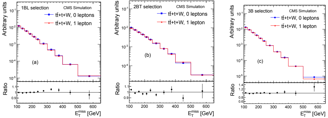
Figure 8: The distributions of E_T^{\text{miss}} in simulated events selected with the (a) 1BL, (b) 2BT, and (c) 3B requirements, except for the requirement on E_T^{\text{miss}} . The square (triangle) symbols show the results for signal (single-lepton SL control) sample events. The small plots below the main figures show the ratio of the signal to SL sample curves. The event samples include t\bar{t} , W+jet, and single-top-quark events.
