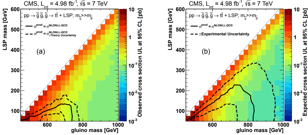
Figure 14: (a) The 95% CL observed cross section upper limits (UL) for the T1tttt SMS model, based on the nominal method to evaluate the top-quark and W+jets background. For each point, the selection that provides the best expected cross section limit is used (the best selection is virtually always 3B). The solid contour shows the 95% CL exclusion limits on the gluino and LSP masses using the NLO+NLL cross section for new physics. The dashed contours represent the theory uncertainties. (b) The corresponding expected limits. The dashed contours represent the uncertainties on the SM background estimates.
