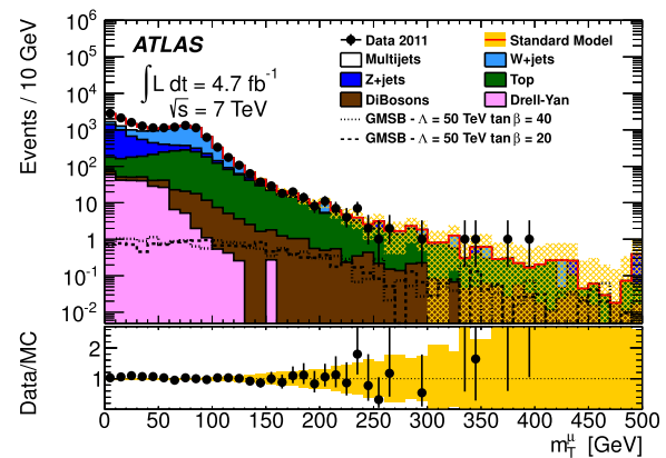
(a) m_T^{\tau+\mu} distribution for the τ+μ final state.
