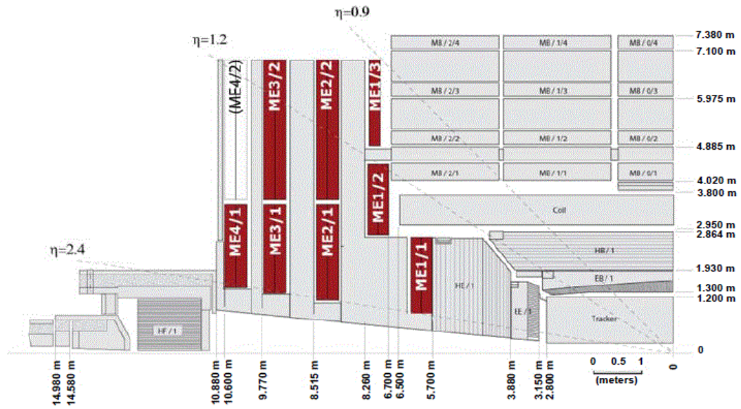
Figure 3.9: Cathode Strip Chamber Geometry in RZ plane. The CSCs are in red, while the DT and magnetic return yoke are in grey. Figure taken from [4].
