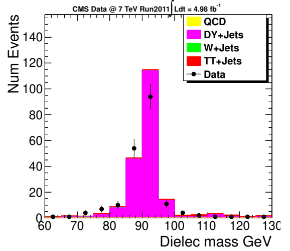
Figure 5.41: Dielectron mass distribution for events with two oppositely signed electrons with 4 jets and HT > 500 .
