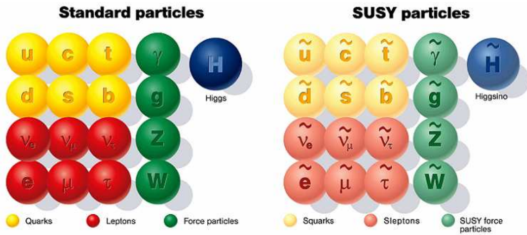
Figure 4.4: Particles of the SM and SUSY. Standard Model particles are shown on the left and SUSY particles are shown on the right with the tilde on top of them. Note that these partnerships are not 1 to 1 since the number of degrees of freedom must remain constant. Figure taken from [10].
