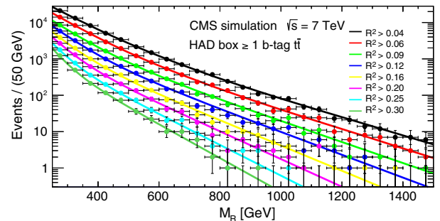
FIG. 31 (color online). The M_R distributions for different values of R^2_{\min} for t\bar{t} simulated events in the HAD box with the requirement of \geq 1 b -tagged jets. The curves show the results of fits of a sum of two exponential distributions.
