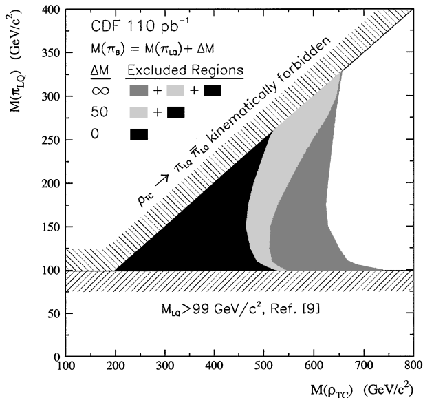
FIG. 2. The 95% C.L. exclusion regions in the M(\pi_{LQ}) - M(\rho_T) plane. The three shaded areas correspond (from left to right) to technipion mass splitting values of 0, 50 \text{GeV}/c^2 , and \infty , respectively.
