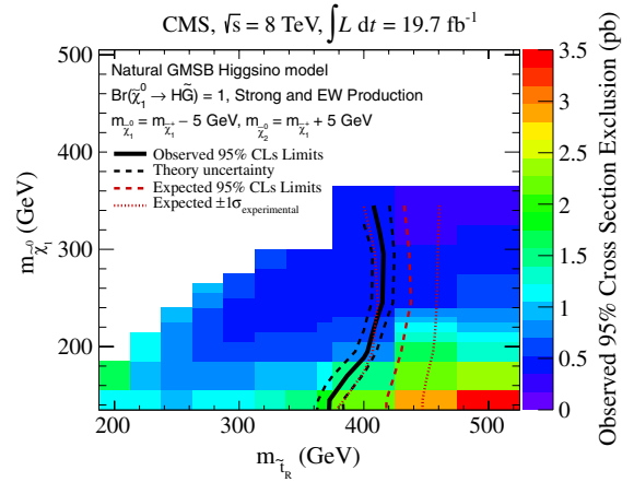
FIG. 4 (color online). Limits on SUSY production cross sections for different top squark and Higgsino masses. The regions to the left of the contours are expected (thick dashed red or gray curves) and observed (solid black curves) to be excluded at the 95% level. Black dashed curves reflect the theoretical uncertainty on the cross section. Red dotted curves correspond to 1 standard deviation in expected sensitivity.
