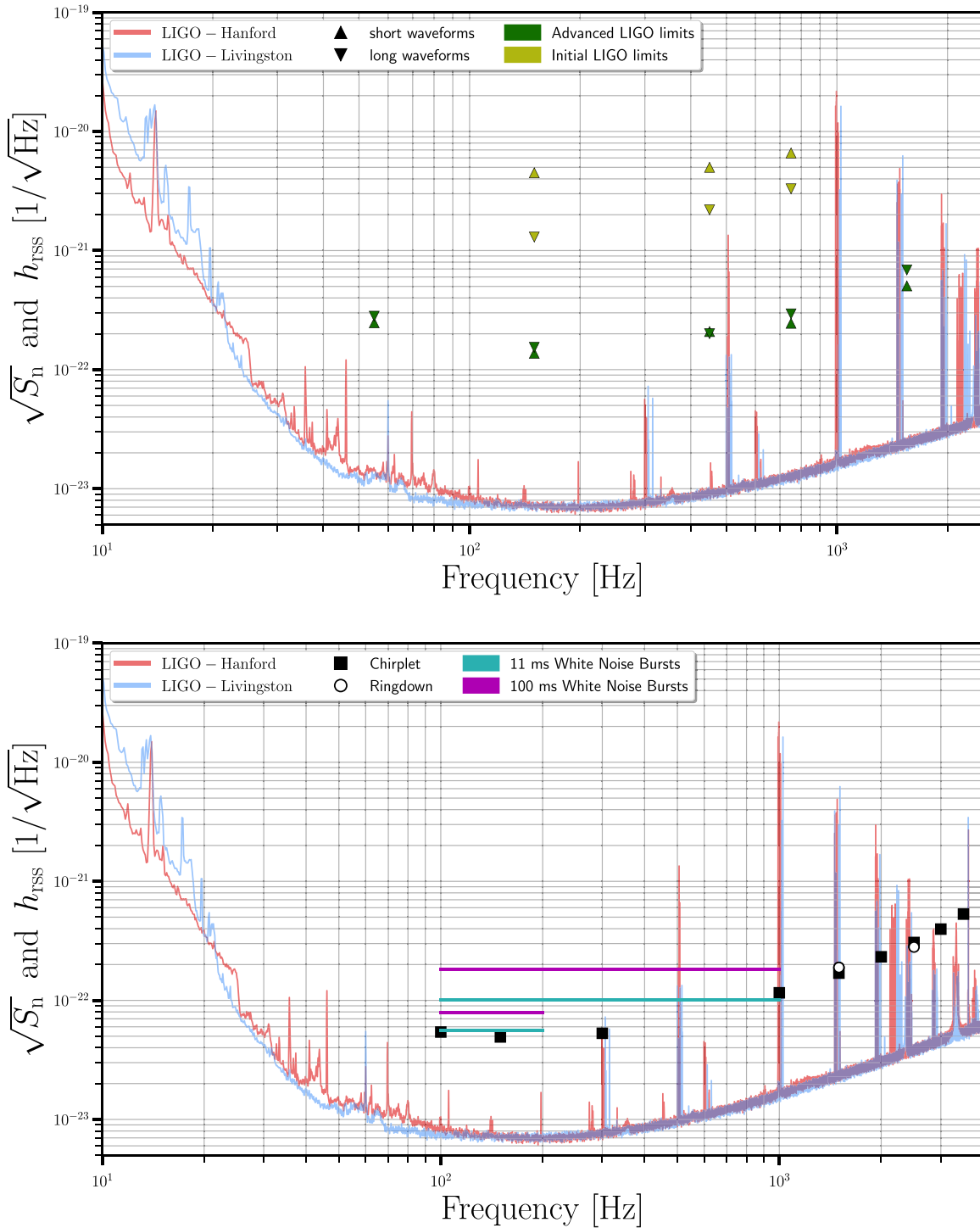
Figure 3. Upper limits for the the intermediate-duration search (above) and short-duration search (below), along with the sensitivity of the detectors. We plot h_{r_{95}} at 90% detection efficiency for the intermediate-duration search here to allow direct comparison to published figures for the previous search in initial LIGO (Quitow-James et al. 2017). Short-duration limits are for 50% efficiency as before. The advanced-duration limits are for the February 25 burst from SGR 1806–20 during the second observing run, and detector sensitivity is calculated from data during the analysis window. The data used to create this figure are available.
