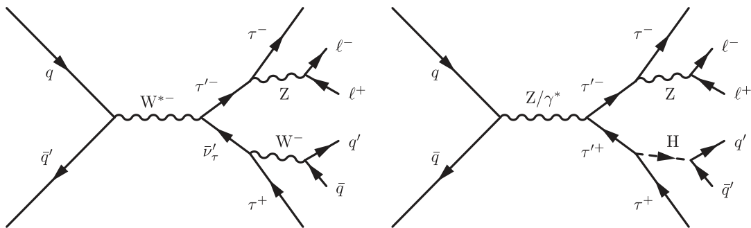
FIG. 1. Two illustrative leading-order Feynman diagrams for associated production of \tau' with a \nu'_\tau (left) and for pair production of \tau' (right) and possible subsequent decay chains that result in a multilepton final state.
