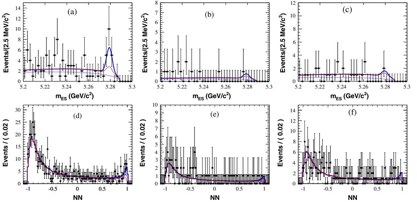
FIG. 8 (color online). Projections on m_{ES} (a, b, c) and NN (d, e, f) of the fit results for DK^+ (a, d), D_{D\pi^0}^*K^+ (b, e) and D_{D\gamma}^*K^+ (c, f) WS decays, for samples enriched in signal with the requirements NN > 0.94 ( m_{ES} projections) or 5.2725 < m_{ES} < 5.2875 \text{GeV}/c^2 ( NN projections). The points with error bars are data. The curves represent the fit projections for signal plus background (solid), the sum of all background components (dashed), and q\bar{q} background only (dotted).
