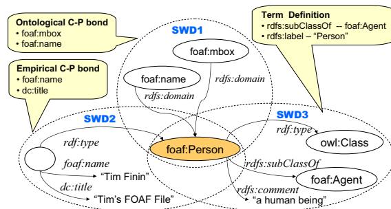
Figure 9: Class definition and class-property bond of foaf:Person
