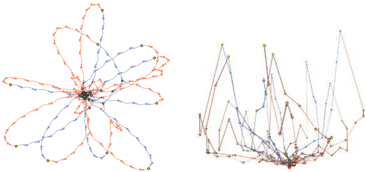
(b) Salomon function D = 3 , SP = 0 .
