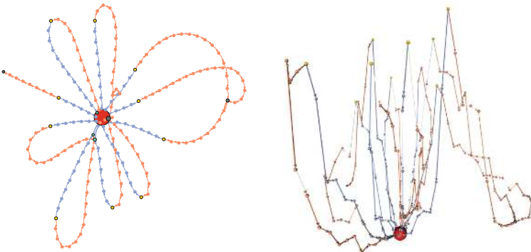
(c) Schwefel 2.26 function D = 5 , SP = -1 .
