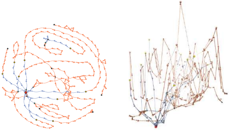
(a) Rana function D = 3 , SP = -1 .
